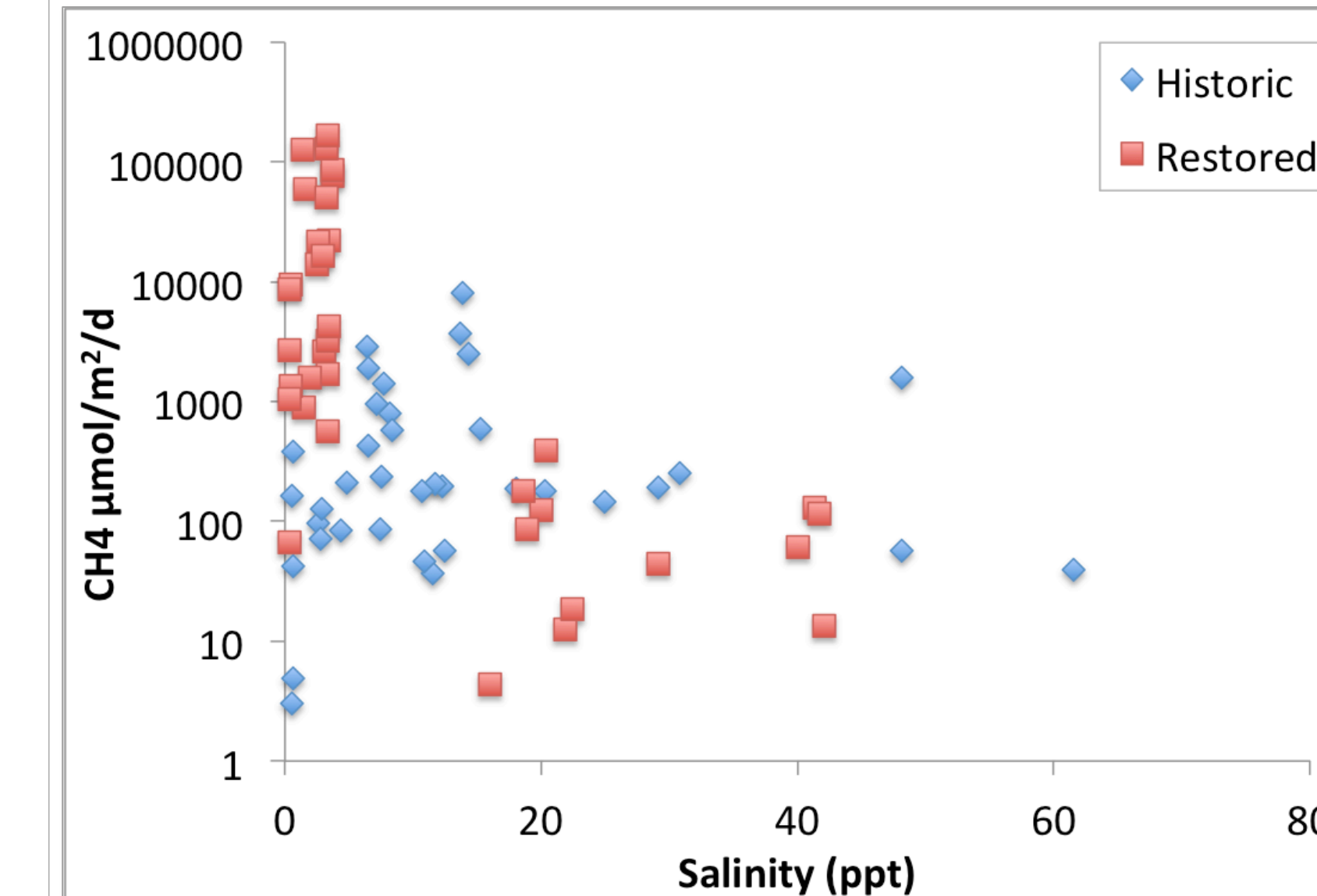
Figure 6. Methane production versus salinity for historic and restored wetlands.
