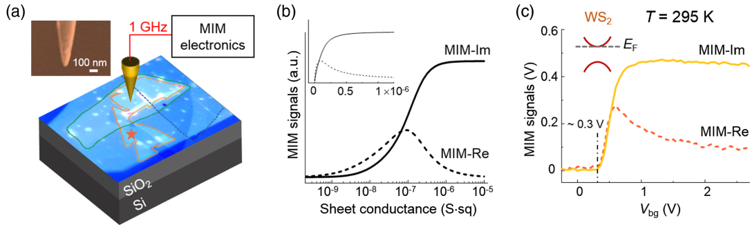
FIG. 2. (a) Schematic diagram of the TF MIM measurements on the \text{WS}_2/\text{WS}_2 heterobilayer device. The inset shows the SEM image of the etched tungsten tip. (b) FEA simulated MIM signals as a function of the sheet conductance of the buried TMD layers. The inset shows the same plot in the linear scale. (c) Measured room-temperature MIM signals on the \text{WS}_2 monolayer [orange star in (a)] as a function of the back-gate voltage. The black dash-dotted line indicates the charge-neutral point for electrons at \sim 0.3 V, where the Fermi level resides at the conduction band minimum (inset).
