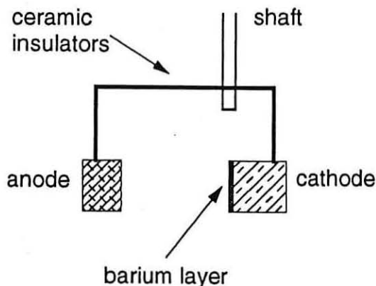
Figure 1. Schematic of the cathode and anode.
