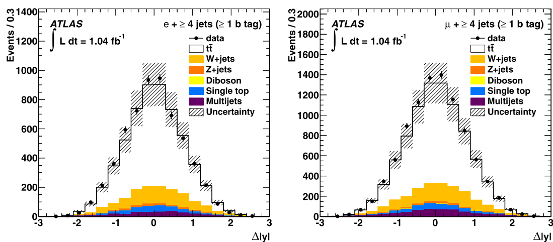
Fig. 3 The measured \Delta|y| distribution before unfolding for the electron channel ( left ) and for the muon channel ( right ) after b -tagging is applied. Data ( points ) and Monte Carlo estimates ( solid lines ) are represented. The multijet background and the normalisation of the
