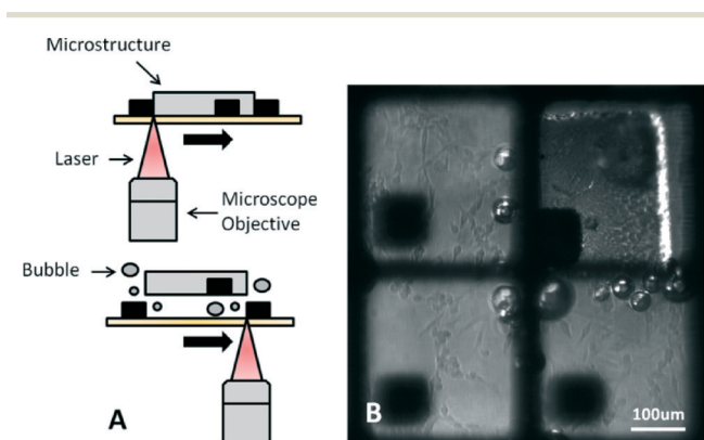
Fig. 4 Ejection of micropallets from gold thin film substrate. A) Schematic of the bubble assisted release of micropallets with a multiphoton laser. B) Image taken with a confocal microscope mid-ejection. Partial release of the structure on the top right of the image can be observed along with the formation of bubbles. Rat208F cells adhered to the surface of surrounding structures were unaffected by the ejection process.
