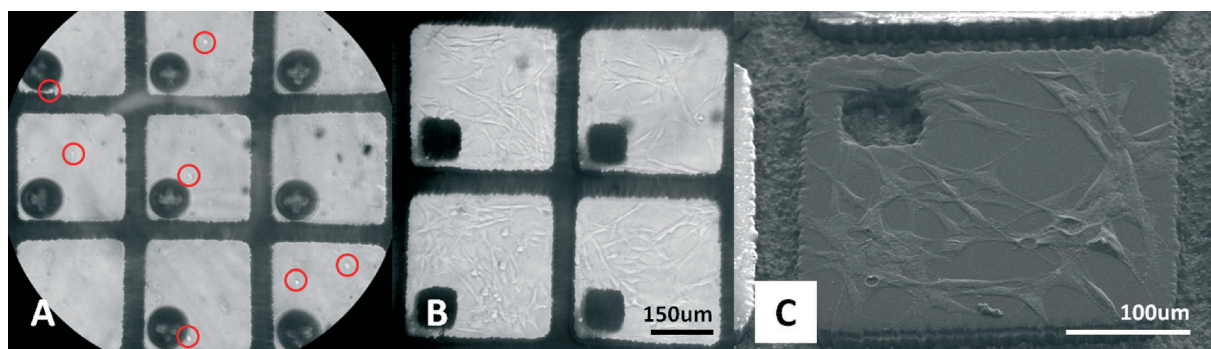
Fig. 3 The capture and growth of cells on magnetic micropallet arrays. A) Cells seeded on micropallets. Individual cells are circled in red. Air bubbles capture within via holes and the borders surrounding the structures constrained cells to the transparent surfaces of the arrays. B) Rat208F cells grown to confluence on micropallets. C) Scanning electron microscope image of an individual micropallet with fixed rat208F cells.
