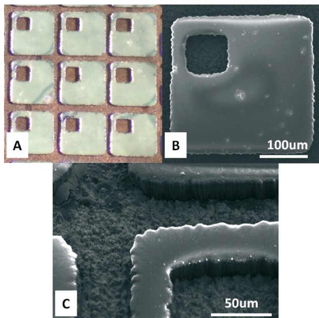
Fig. 2 Magnetic cell colony arrays electroplated with 500 nm gold/30 \mu\text{m} nickel/500 nm gold. A) Section of a completed array revealing the top layer of gold coated on both the borders surrounding the structures and within their via holes. B) Scanning electron microscope (SEM) image of an individual magnetic micropallet. C) SEM image of a corner section of an individual pallet. The metal plating can be seen rising to 30 \mu\text{m} along the sides of the 50 \mu\text{m} tall structure.
