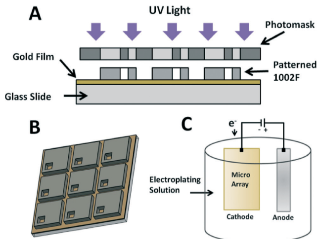
Fig. 1 Fabrication of micropallet arrays containing via holes on gold thin films. A) Schematic of the photolithographic patterning process of the micropallet array. B) Representation of patterned structures. Regions of the gold thin film are exposed within each micropallet through a via hole for the electroplating of ferromagnetic nickel cores. C) Schematic of electroplating setup. Microarrays are linked to a power source and immersed in an electroplating solution along with an anode. Electroplating occurs on all exposed conductive surfaces of the micropallet array.
