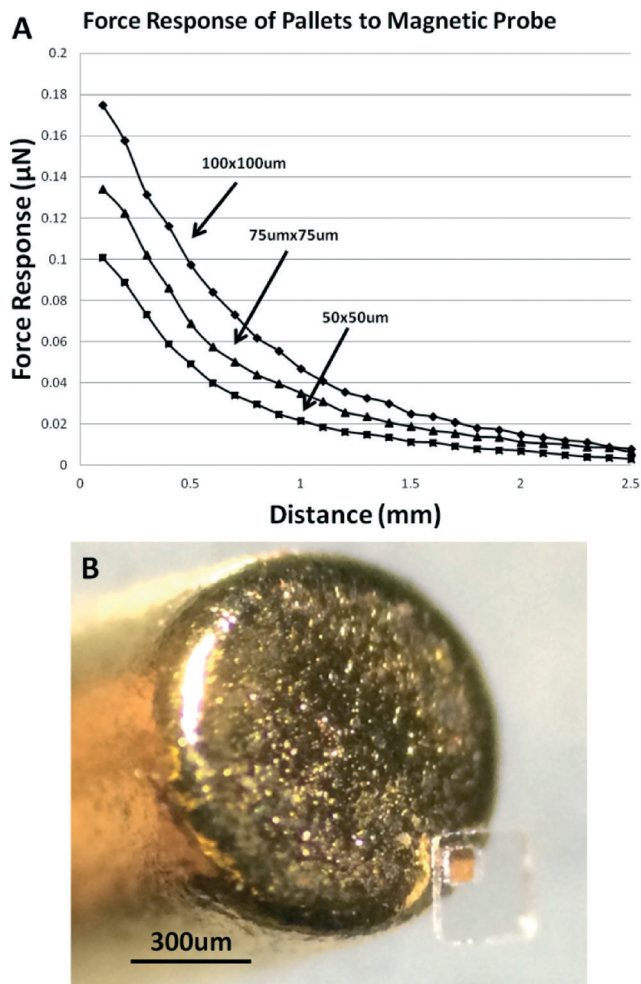
Fig. 6 Magnetic properties of micropallets. A) Force response of three different ferromagnetic core sizes. B) Individual captured micropallet on a 1 mm diameter neodymium magnet. The magnet was unshathed (as shown) during micropallet force response experimentation in order to record the maximum force response to the 225 Gauss magnetic field.
