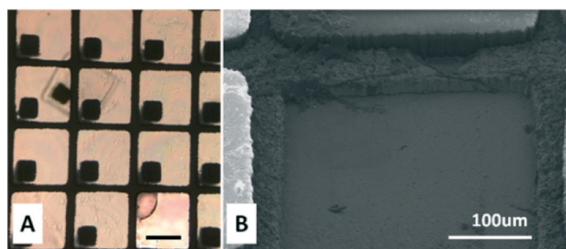
Fig. 7 Released micropallet with adhered cell colony. A) Phase contrast image of a released pallet resting on top of surrounding structures. The structure's original location can be observed on the bottom right of the image. The scale bar is 200 \mu\text{m} and located on the image at the site of the released pallet. B) Scanning electron microscope image of the pallet ejection site. The metal walls which previously surrounded the structure are maintained during the ejection process.
