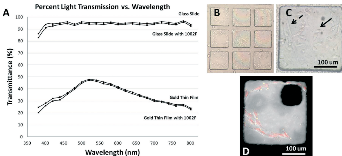
Fig. 5 Light transmission properties of gold thin films deposited to glass microscope slides. A) Chart comparing transmittance of glass slides, glass slides coated with a 50 \mu\text{m} layer of 1002F photoresist, glass slides coated in a gold thin film, and glass slides coated in a gold thin film with a 50 \mu\text{m} layer of 1002F photoresist to represent the final transmittance properties of the cell colony arrays. B) Image of an array of 1002F micropallets on a gold thin film with cells grown on their surfaces. Each structure is a 270 \times 270 \mu\text{m} square with a 50 \mu\text{m} height. C) Individual 270 \times 270 \times 50 \mu\text{m} micropallet on gold with a mixture of seeded HeLa and NIH 3T3 WT cells. The dotted arrow is pointing to a 3T3 cell and the solid arrow is pointing to a HeLa cell. D) Magnetic microstructures with 7AAD (red) and Annexin V (yellow) stained rat208F cells.
