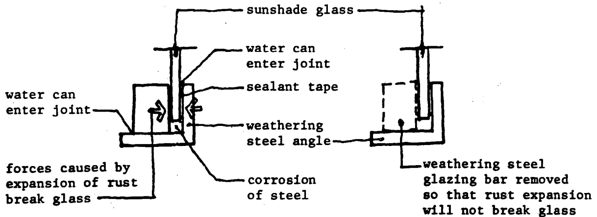
b) Section with bar removed
