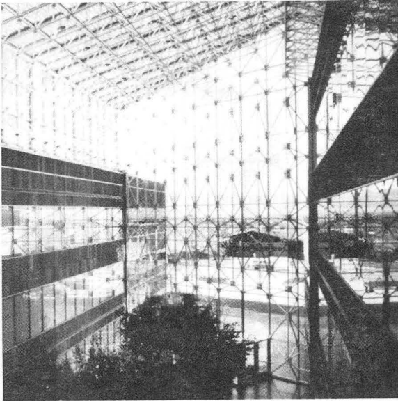
Figure 8. View of atrium interior.
