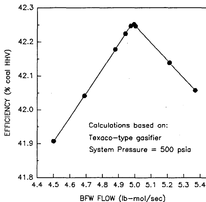
Figure 4-3: Effect of Boiler Feed-Water Flow on System Efficiency
