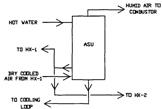
Figure 7-3-b: Configuration with Side Stream
