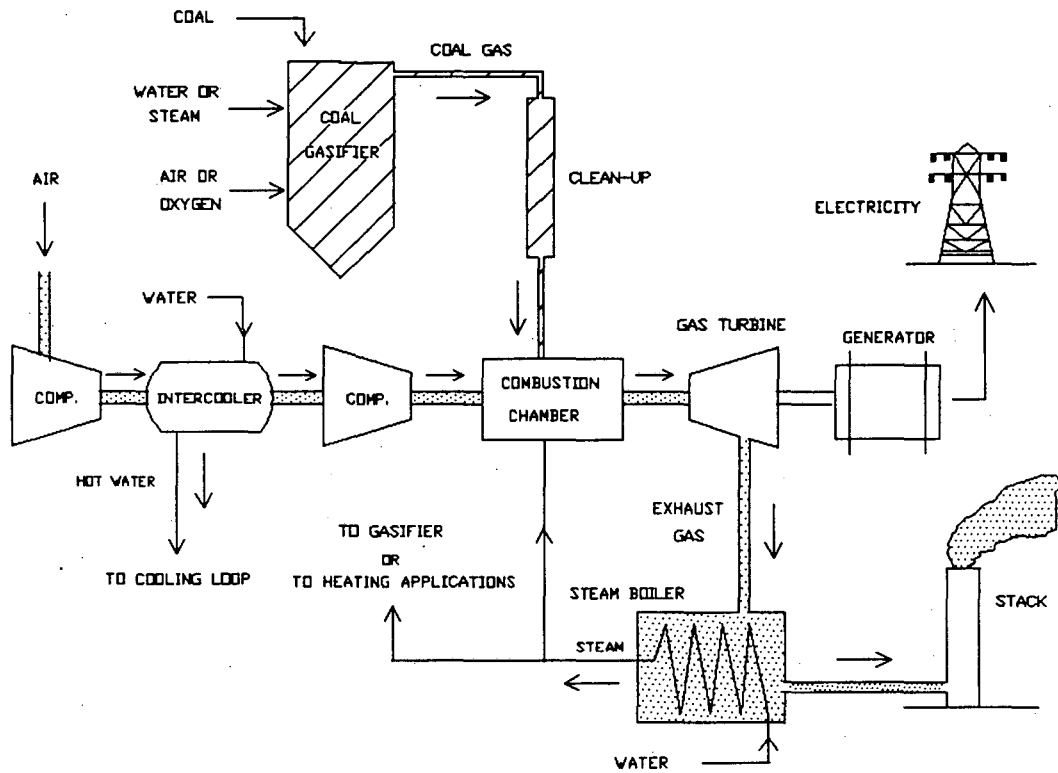
Figure 1-3: Intercooled Steam-Injected Gas (ISTIG) Turbine System
