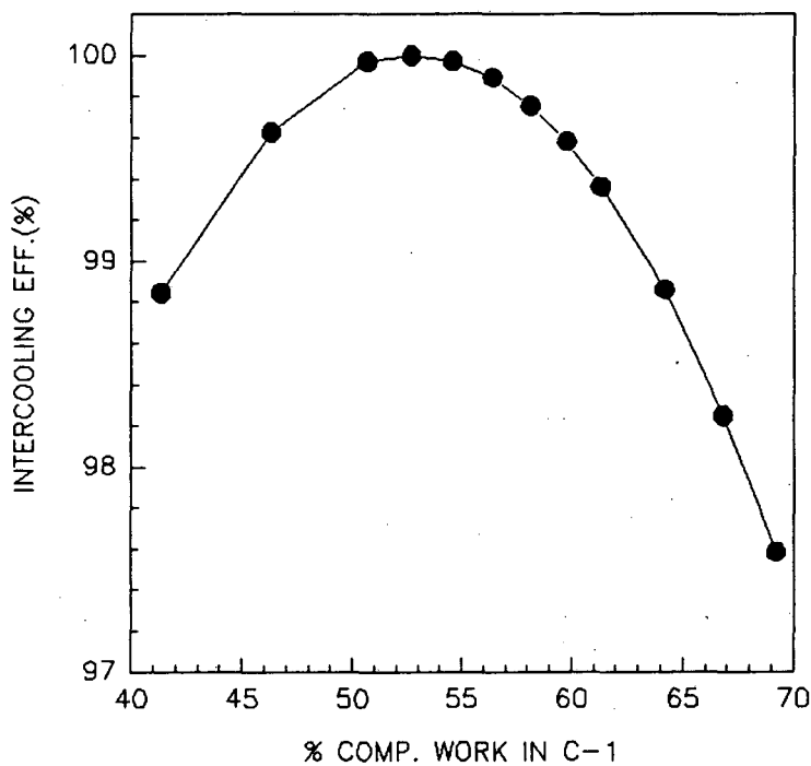
Figure 3-2: Intercooling Efficiency
