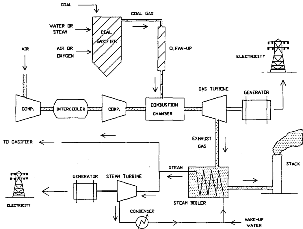
Figure 1-2: Combined Cycle
