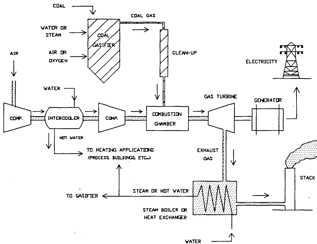
Figure 1-1: Cogeneration
