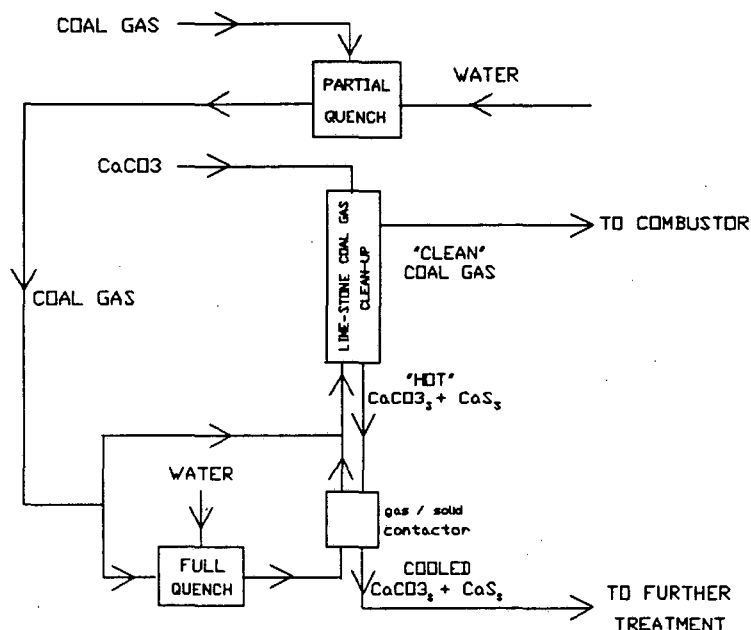
Figure 3-3: Clean-Up Section
