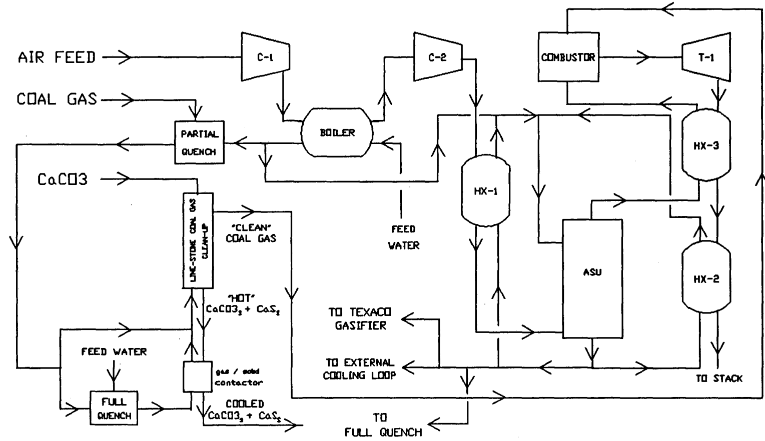
Figure 3-5: Improved Heat Recovery Method for Coal-Gas Combustion Turbine Systems using Texaco Gasifying Process
