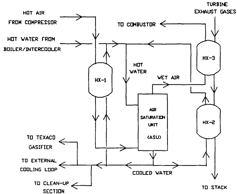
Figure 3-4: Heat-Recovery Section
