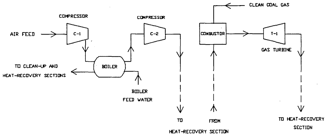
Figure 3-1: Core Section
