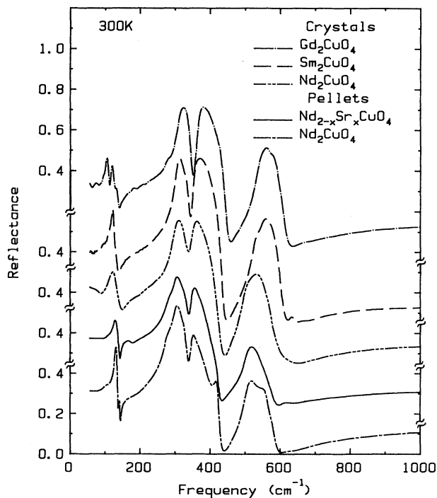
FIG. 2. Infrared reflectance for three single crystals and two pellet samples for a series of rare-earth substitutions (the curves have been offset by a constant for ease of viewing).
