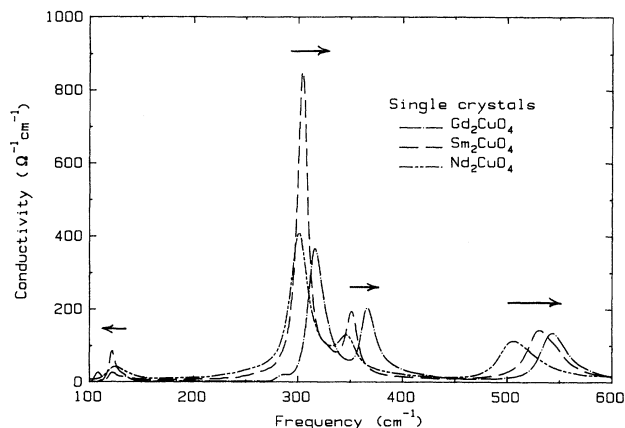
FIG. 4. Frequency-dependent conductivity for crystal samples as obtained from Kramers-Kronig analyses. Arrows indicate shift direction with increasing R mass.
