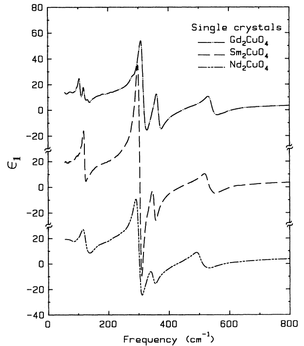
FIG. 6. The real part of the dielectric function \epsilon_1(\omega) for single-crystal samples plotted with the zeros offset for ease of comparison.
