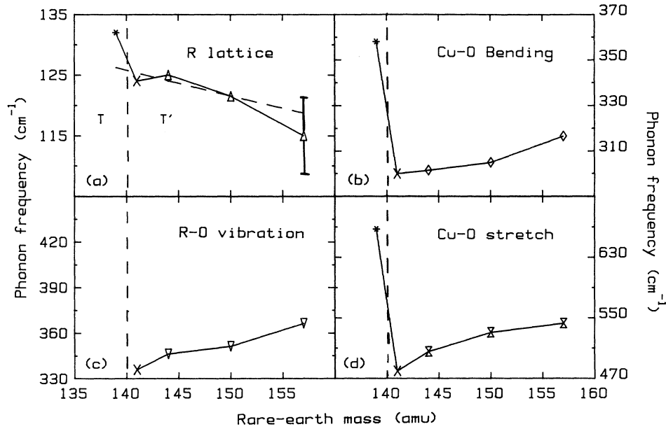
FIG. 5. Center frequency as a function of rare-earth mass for each of the in-plane ir active modes at room temperature. Data for Pr ( T=10 K) by Crawford et al. (Ref. 13) ( \times ) and for La ( T=300 K) by Collins et al. (Ref. 8) ( * ) is also shown.
