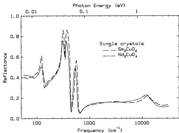
FIG. 3. Reflectance in the infrared and visible for crystals of \text{Sm}_2\text{CuO}_4 and \text{Nd}_2\text{CuO}_4 .
