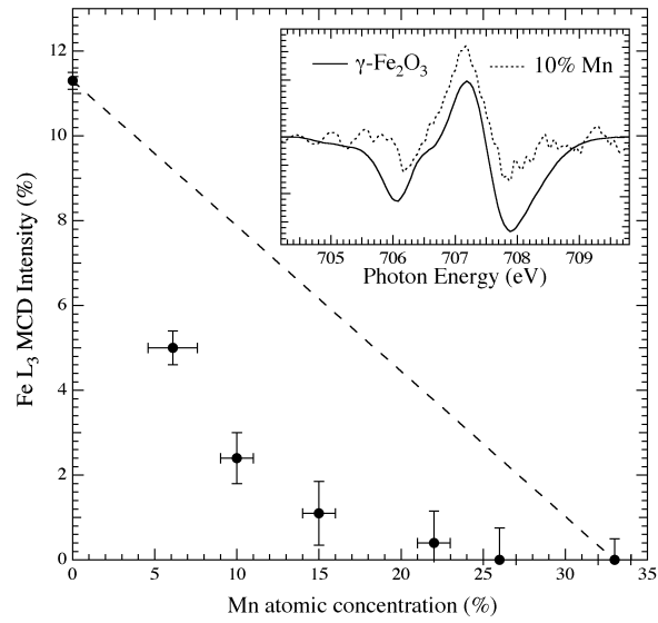
FIGURE 2: Fe L 3 XMCD intensity as a function of Mn concentration (data – filled circles, model – dashed line). INSET: Normalized Fe L 3 XMCD spectra for 0% Mn doping and 10% Mn doping.
