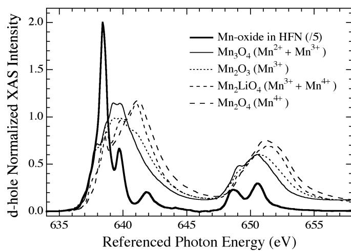
FIGURE 1: Mn L 23 XAS spectra for Mn doped at 33% into 6.7 nm diameter iron oxide nanoparticles (heavy line) and various Mn oxide reference powders.
