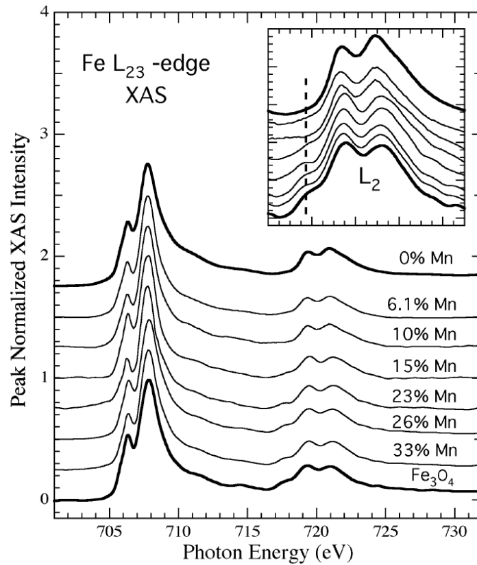
FIGURE 3: Fe L 23 -edge XAS as a function of Mn concentration. The heavier lines are the spectra for 0% Mn or \gamma -Fe 2 O 3 in HFN (upper) and the reference Fe 3 O 4 (lower). INSET, Fe L 2 -edge showing the growth of the shoulder and the redistribution of spectral weight between the two L 2 peaks.
