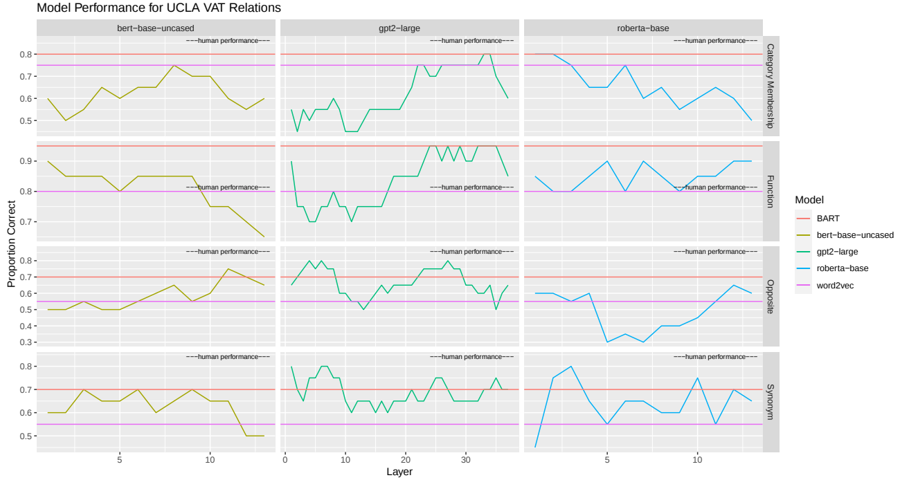
Figure 3: Model Comparisons with Human Accuracy in Solving Verbal Analogy Problems Accuracy of each model (and each layer of LLMs) for problems in the UCLA VAT based on each of four relation types. Mean human accuracy from Lu et al. (2019) is indicated at right side in each panel.
