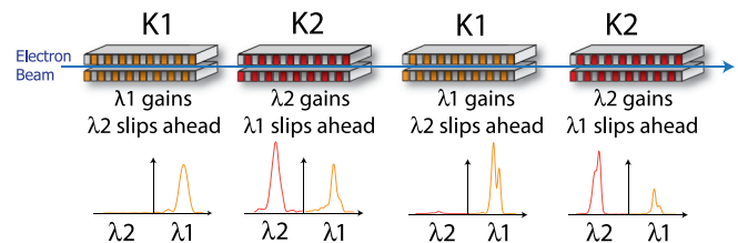
FIG. 1 (color online). Schematics of a gain-modulated FEL. The undulator parameter K varies periodically along the FEL beam line. In each undulator section, the resonant wavelength is amplified exponentially while the nonresonant wavelength slips ahead of the electrons without amplification. The resulting spectra exhibit multiple spectral lines.
