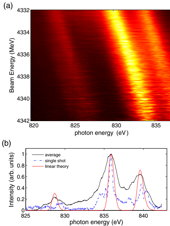
FIG. 3 (color online). (a) Average intensity as a function of beam energy and photon energy for an undulator periodicity of 2 undulator modules. (b) Average spectrum (black line) and single-shot spectrum (dashed blue line) for a beam energy of 4334 MeV. For comparison, the spectrum predicted from the linear theory is plotted as a red line.
