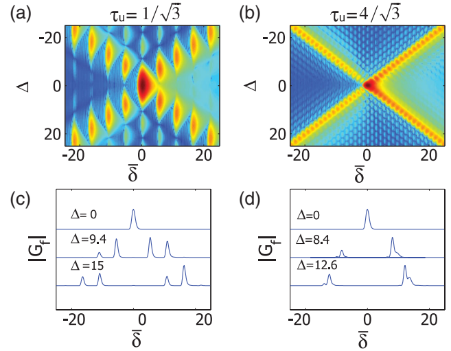
FIG. 2 (color). Gain curve (logarithm of the gain function G_f ) as a function of the average detuning \bar{\delta} and the undulator detuning \Delta (upper images) for an undulator periodicity of two power gain lengths (a) and eight power gain lengths (b). (c),(d) Linear plots of the gain function for three different values of \Delta .
