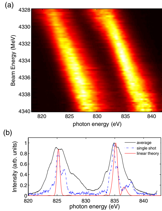
FIG. 4 (color online). (a) Average intensity as a function of beam energy and photon energy for an undulator periodicity of 6 undulator modules. (b) Average spectrum (black line) and single-shot spectrum (dashed blue line) for a beam energy of 4334 MeV. For comparison, the spectrum predicted from the linear theory is plotted as a red line.
