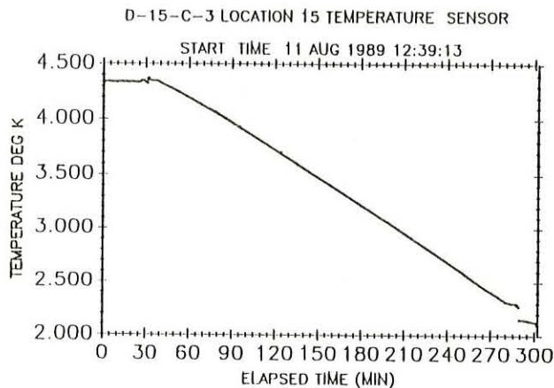
Figure 3. Temperature Record of Dipole D-15C-3
