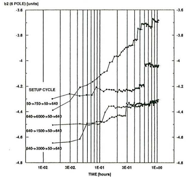
Figure 10. Sextupole Decay of D-15B-2 at 640A
