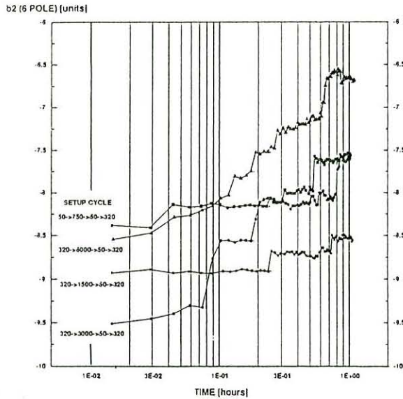
Figure 9. Sextupole Decay of D-15B-2 at 320A
