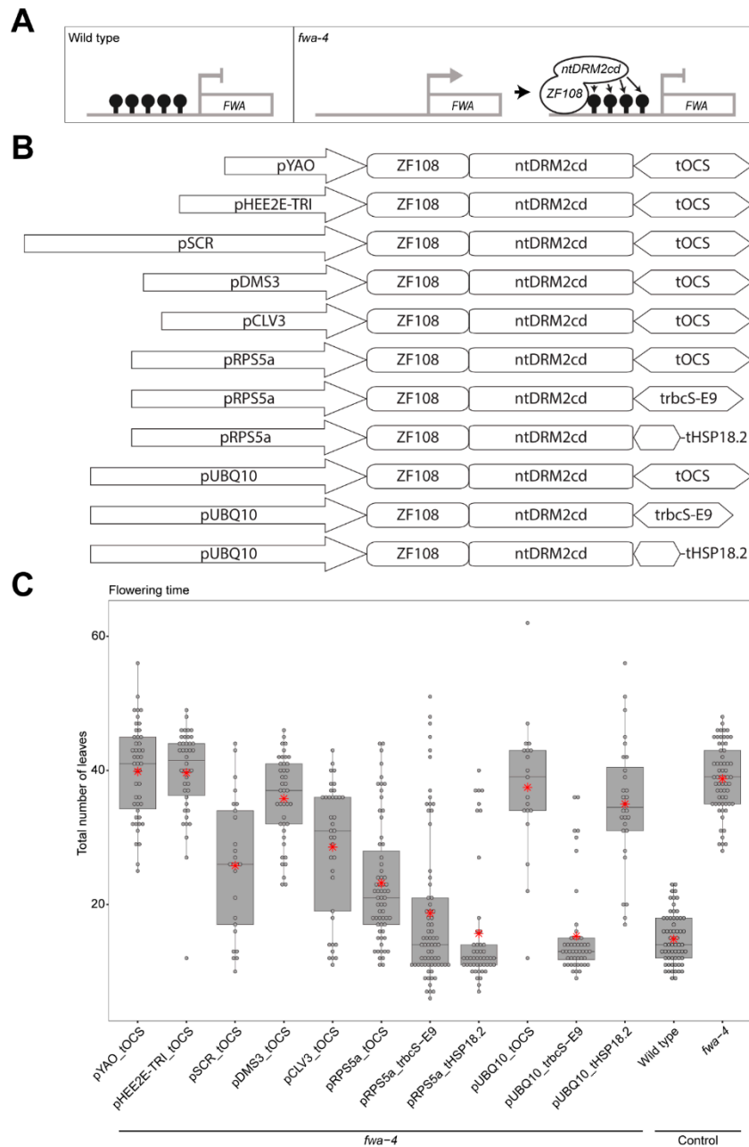
Figure 1. Use of different promoter and terminator combinations can change the efficiency of targeted DNA methylation. (A) Schematic representation of the FLOWERING WAGENINGEN ( FWA ) promoter region in wild type (where the promoter region is methylated and FWA gene expression is silenced), and the FWA promoter region in the fwa-4 epiallele (where the promoter region is unmethylated and
