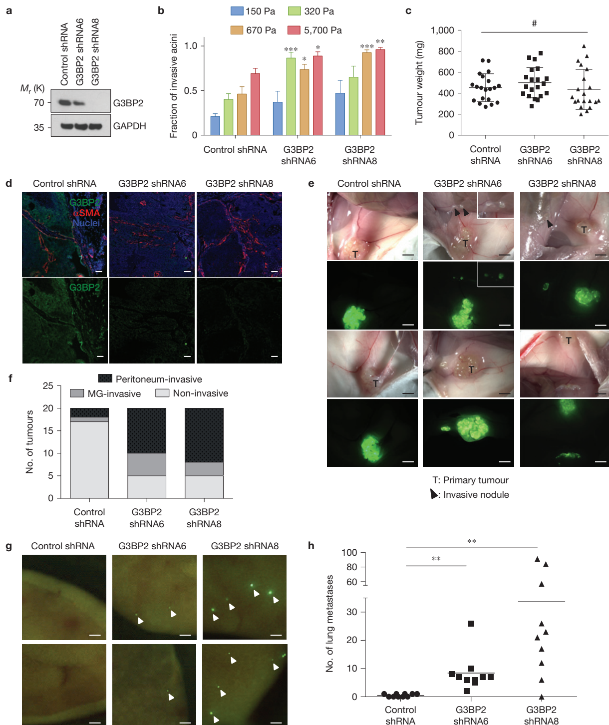
Figure 6 Loss of G3BP2 induces tumour invasion in vivo . (a) Cell lysates from MCF10DCIS cells expressing control or G3BP2 shRNAs were analysed by SDS-PAGE and probed for G3BP2 and GAPDH. Unprocessed original scans of the blots are shown in Supplementary Fig. 7. (b) Quantification of invasive acini formed by MCF10DCIS cells expressing control or G3BP2 shRNAs cultured in 3D culture with varying rigidities for 5 days (*, P < 0.05 ; **, P < 0.01 ; ***, P < 0.001 , unpaired two-tailed t -test with Welch's correction, n = 50 acini per experiment, 3 independent experiments; error bars denote s.e.m.). (c) Tumour weight of MCF10DCIS xenograft tumours expressing control or G3BP2 shRNAs (#, not statistically significant, unpaired two-tailed t -test with Welch's correction, n = 20 tumours from 10 mice per group,
