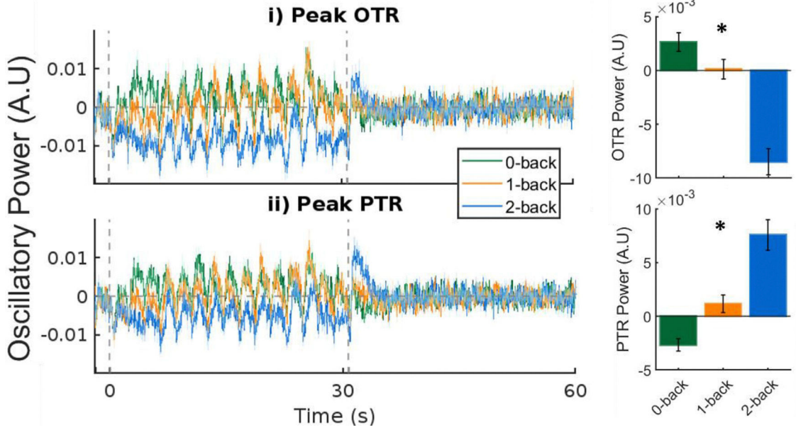
Fig. 5. Dorsal attention network. Group-averaged beta timecourses across the whole dorsal attention network (DAN), at locations of peak activity during the OTR (i, 0.5 – 29.5 s) and PTR (ii, 31.5 – 33.5 s) time-windows. Bar charts on the right show average power in the corresponding time windows across conditions. Activity during both time windows modulated significantly ( p < 0.05 , rm-ANOVA) with task condition, denoted with an asterisk (*). Post-hoc t-tests showed that all pairs of conditions varied significantly ( p < 0.05 , t-test) in both time-windows. Shading around timecourses and error bars on bar charts represent standard error over subjects for each measure.
