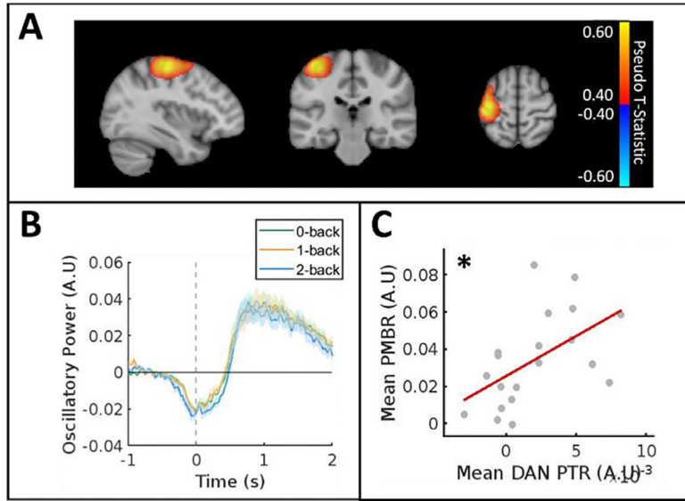
Fig. 6. Post-movement beta rebound. The well-studied beta response to movement in the motor cortex. Panel A shows a T-stat map found by contrasting the PMBR period (0.5 – 1.5 s relative to button press) with the MRBD period (–0.5 – 0.5 s relative to button press) across all conditions. A clear positive peak can be seen in the left (contralateral) motor cortex. Panel B shows the extracted timecourses for each condition, averaged over all correct button presses and over all subjects. The time axis is set such that zero is the time of the button press. The shaded area around each line denoting the standard error over subjects. There were no significant modulations between conditions during the MRBD nor the PMBR. Baselines were removed from timecourses using 48 – 58 s used in Figs. 4, S1 and S3. Panel C shows the relationship over subjects between the mean PMBR with the mean DAN PTR over all conditions. * denotes a significant ( p < 0.05 ) correlation.
