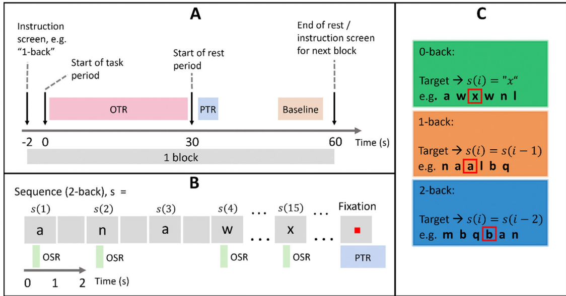
Fig. 1. The n-back paradigm. Panel A : Each block started with an instruction screen at -2 s, which read either “0-back”, “1-back” or “2-back”, indicating the condition that would follow. The task period started at 0 s, lasting for 30 s. The rest period started at 30 s and lasted for 30 s. At 60 s, the instruction screen for the next block was shown. The oscillatory task response (OTR) window (0.5 – 29.5 s), the post-task response (PTR) window (31.5 – 33.5 s) and the baseline window (48 – 58 s) are shown. Panel B shows the timing of the presentation of individual stimuli and indicates oscillatory stimulus response (OSR) window (0.3 – 0.5 s following the start of each stimulus presentation). Panel C shows the three different task conditions, with the red boxes indicating the target letters. Each subject completed a total of 16 blocks of each condition, in a pseudorandom order, spread over two separate runs.
