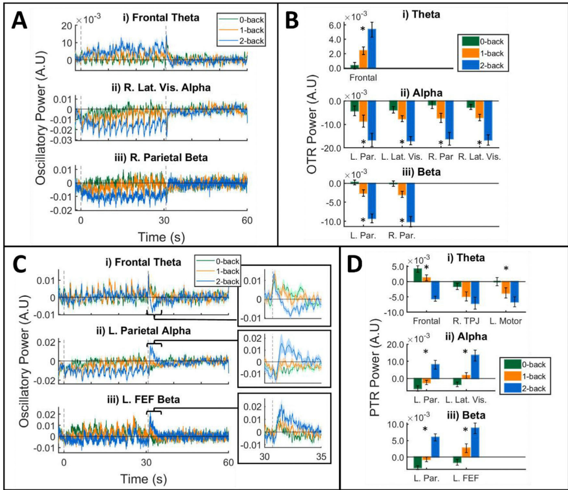
Fig. 4. Group timecourses and average power modulations. Timecourses and bar charts from peak T-stat locations in each frequency band. Panels A and C show group averaged timecourses from representative OTR and PTR locations in each frequency band (other timecourses can be seen in Fig. S1 and S3). Timecourses were averaged during the relevant time windows to give the average power over the time windows for each region which is displayed in the bar charts (panels B [OTR] and D [PTR]). Panels A and B show effects during the OTR window (0.5 – 29.5 s), whilst panels C and D show effects during the PTR window (31.5 – 33.5 s). Bar charts that show significant ( p < 0.05 , rm-ANOVA) change across conditions are marked with an asterisk (*). Shading around timecourses (A and C) and error bars (B and D) denote standard error over subjects for each measure.
