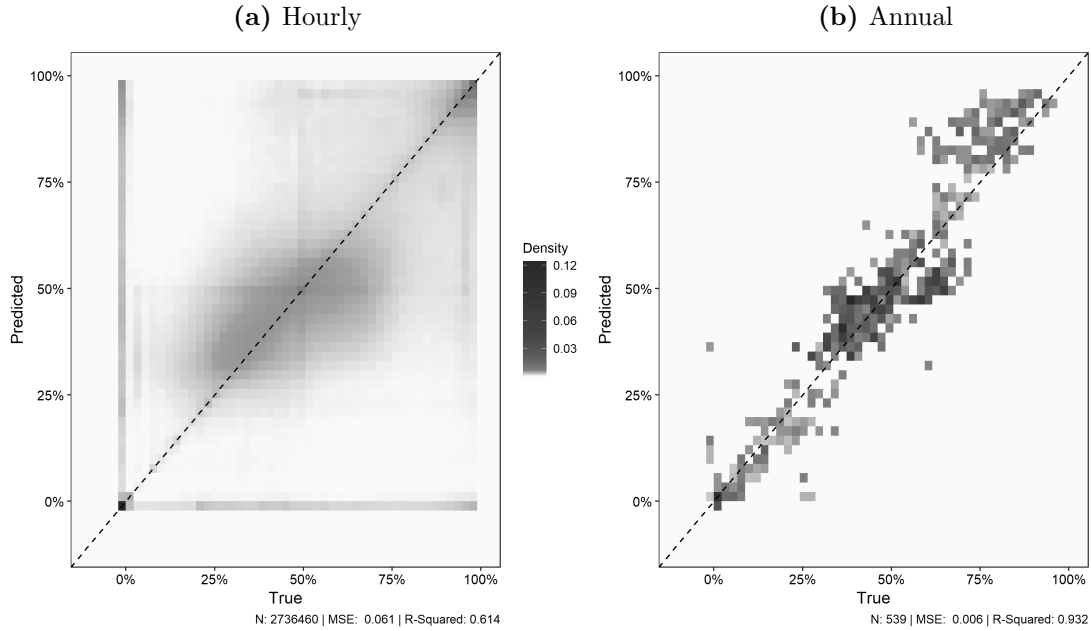
Figure 4: Machine Learning Model Performance: Plant-Level Electricity Production
