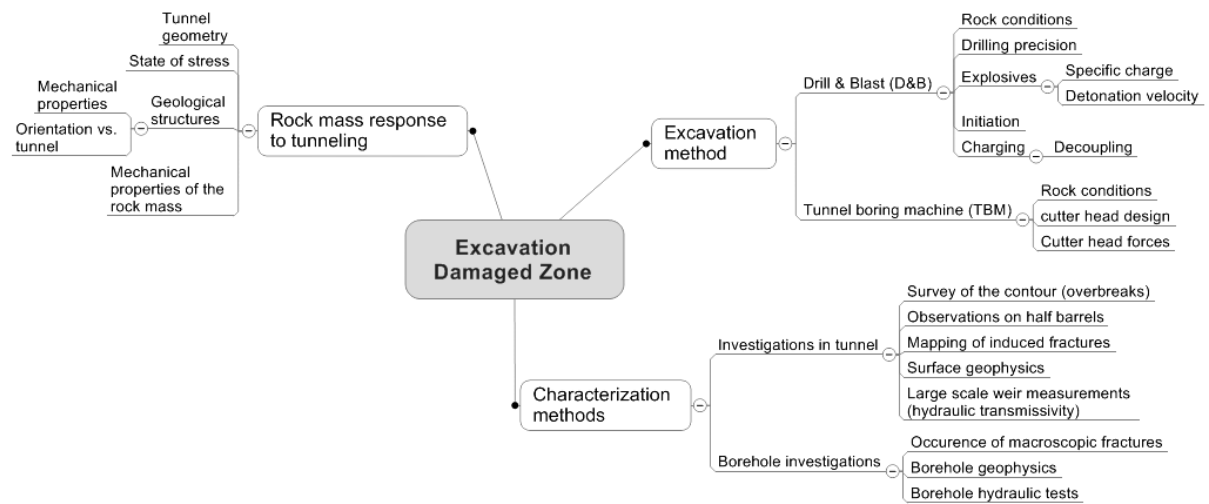
Figure 2: Summary of the factors relating to the rock mass response to tunnelling, the excavation method, and characterisation methods.
