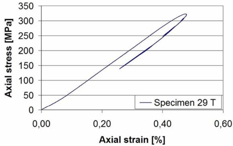
Figure 4: Stress-strain curve (Class II type – does not monotonically increase in axial strain) for the Ävrö granite – which is ultra-brittle.
