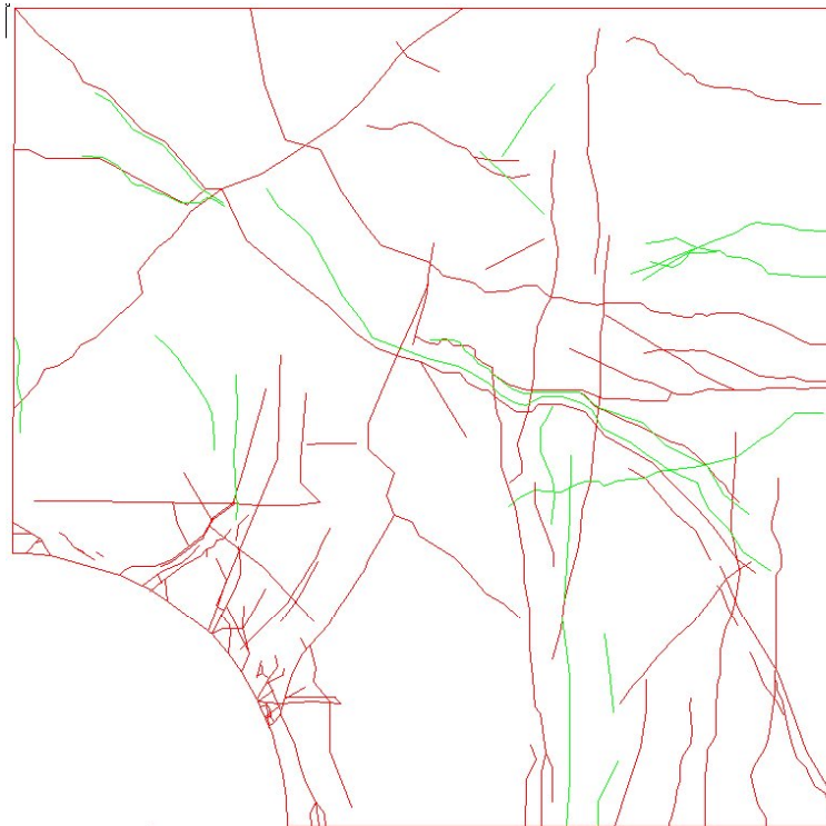
Figure 7: Fracture pattern used as a starting point by each research team. Open fractures are coloured red and filled fractures are green.
