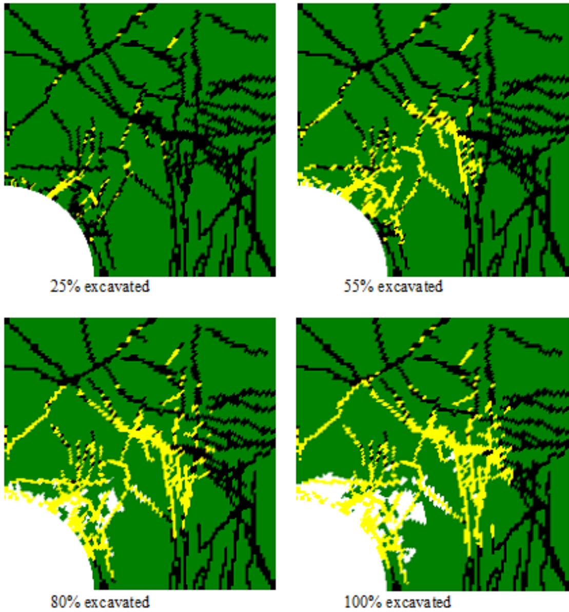
Figure 10: Evolution of failure represented by Mohr-Coulomb yielding in matrix rock (with contours) and fractures (yellow contour) calculated with the CAS2 model.
