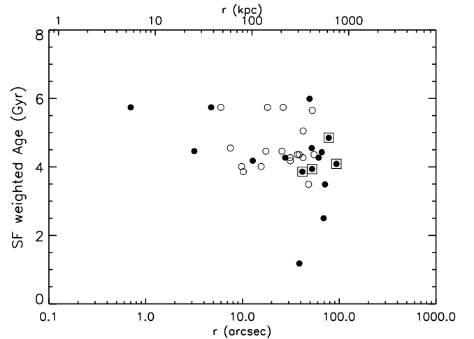
Fig. 12. SF weighted age versus radial distance to the cluster center. Spectroscopic members with [OII] emission or morphologically classified as late-type galaxies are indicated by square symbols.
