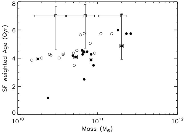
Fig. 11. Photometric masses of the 16 spectroscopic cluster galaxies (filled circles) and 18 “red-sequence” ETGs (open circles) as a function of their star-formation-weighted ages. Spectroscopic members with [OII] emission or morphologically classified as late-type galaxies are indicated by square symbols. Mean error bars corresponding to three mass bins (bin1: m < 4.5 \times 10^{10} M_{\odot} , bin2: 4.5 \times 10^{10} M_{\odot} < m < 1 \times 10^{11} M_{\odot} , bin3: m > 1 \times 10^{11} M_{\odot} ) are shown at the top of the figure.
