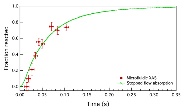
Figure 4. Fractional conversion vs. time using fit parameters extracted from XAS fits (1.4 mM CdSe, 5 mM AgClO 4 , red dots) and stopped flow experiments (1.4 mM CdSe, 6.67 mM AgClO 4 at 1:1 volumetric ratio, green line). Error bars show 95% confidence limits.
