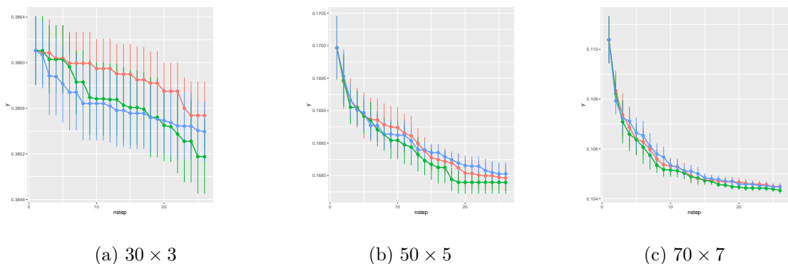
Figure 4.3: Minimization path for 3 methods in the construction of UPDs using DE
