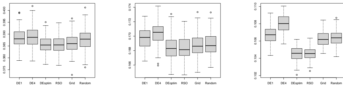
(a) 30 \times 3 as target
