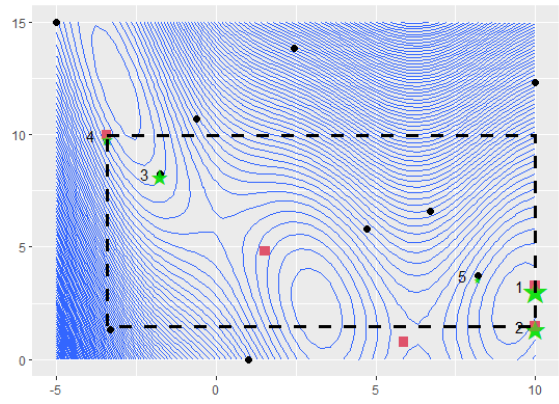
(b) Initial ROI containing the top 30% of points
