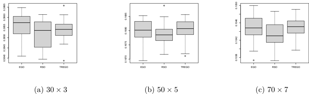
Figure 4.4: Comparison of optimal results from 3 methods
