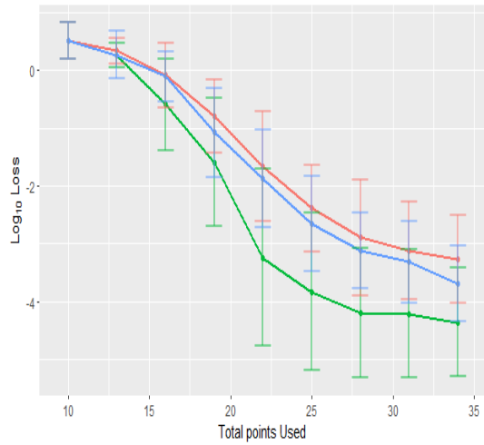
(a) Branin function
