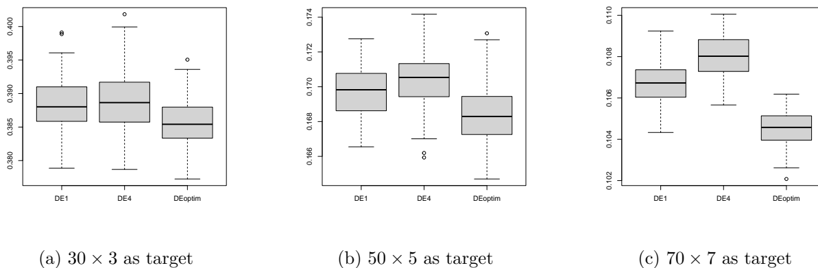
Figure 2.8: Performance of the DE algorithms under three settings: DE1, DE4 and DEoptim (optimal settings)
