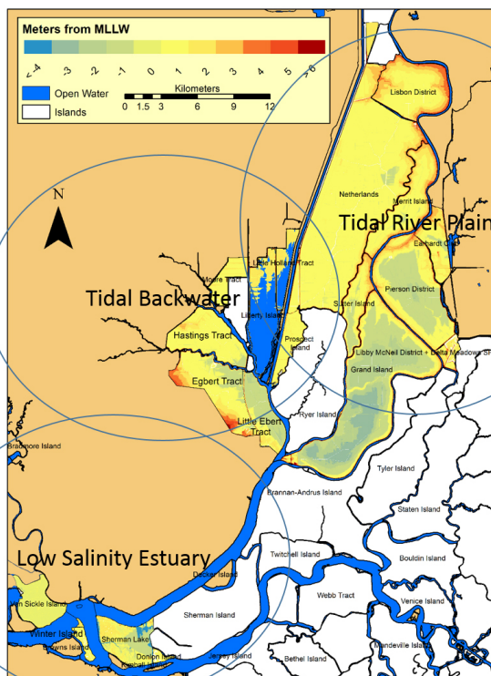
Figure 8 Regions dominated by high-scoring polders on the NSBI
