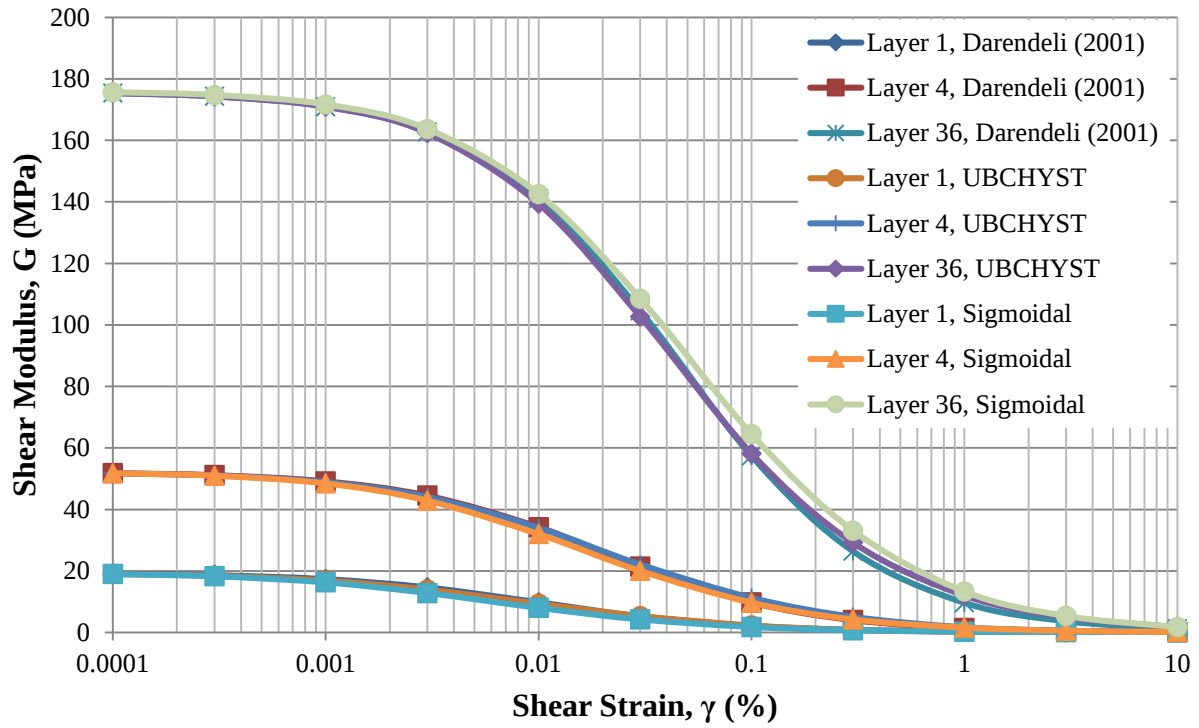
Figure 5.5: Shear modulus degradation vs shear strain
