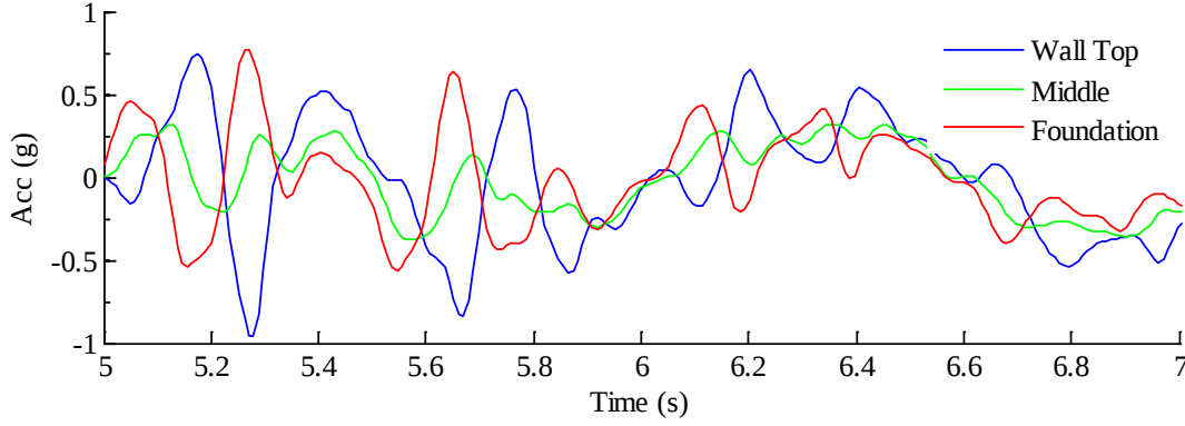
Figure 4.2: Response of basement wall at various depths during Kobe TAK 090-3
