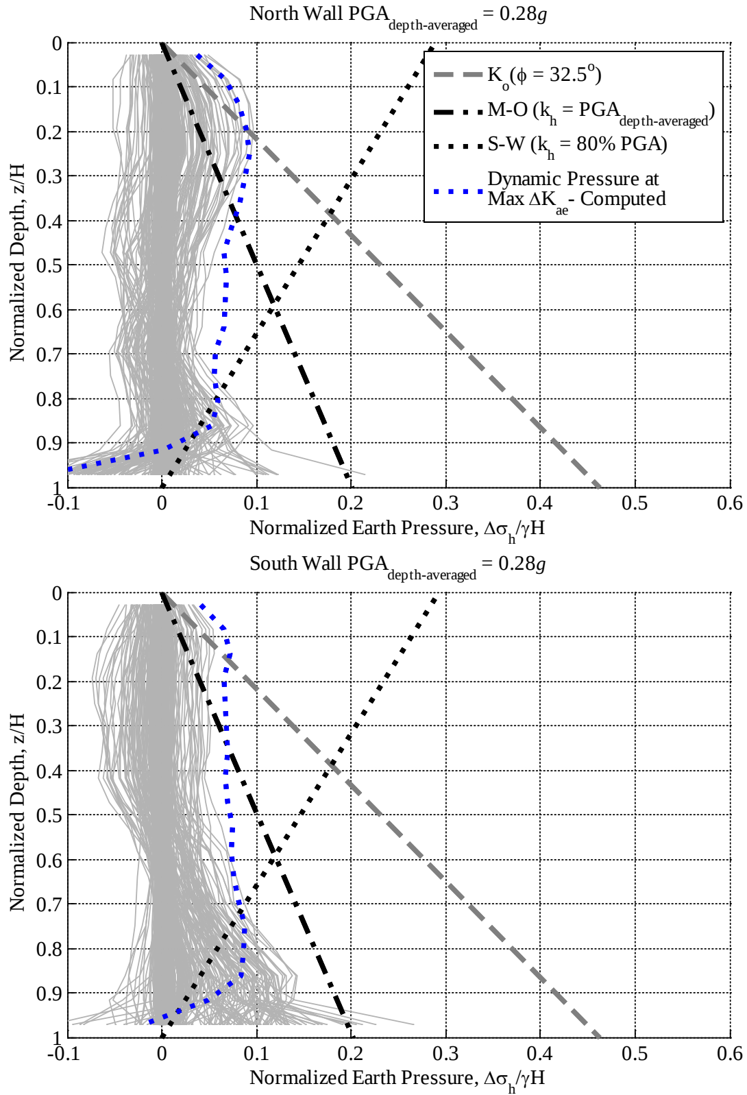
Figure 6.18: Computed normalized dynamic earth pressure distributions at maximum \Delta K_{ae} during Loma Prieta CAP 000 for three level basement; Site Class D
