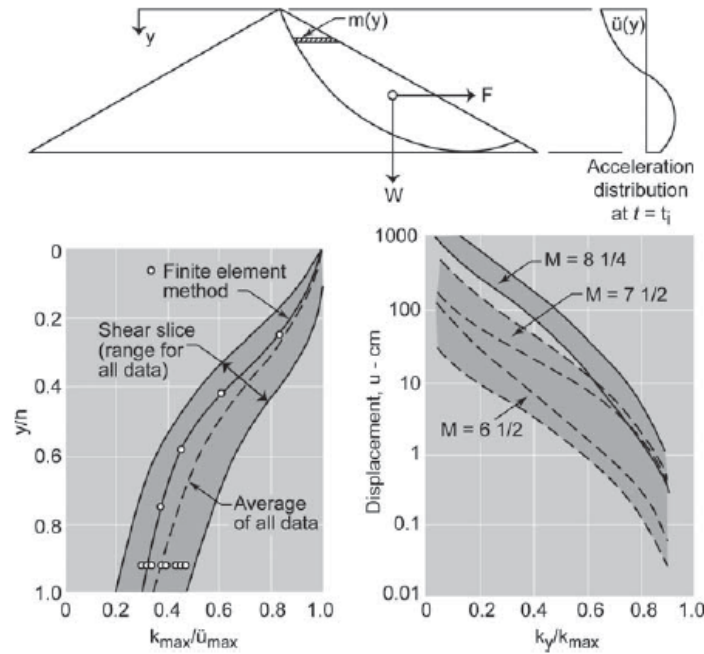
Figure 7.6: Permanent seismic deformation charts from Makdisi & Seed (1978) (adapted from Anderson et al. (2008))
