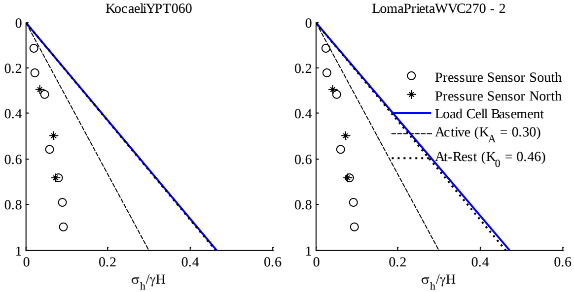
Figure 4.5: Static earth pressure in basement wall prior to ground motion ( H = 13.47 m, \gamma H \approx 225 kN/m 2 )
