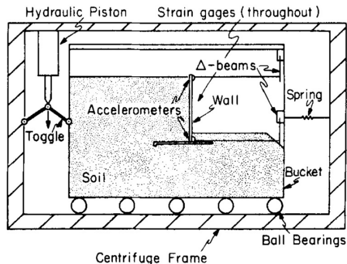
Figure 2.11: Centrifuge experiment setup of Ortiz (1982)
