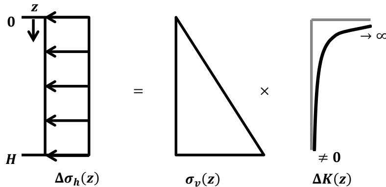
Figure 7.9: Dynamic earth pressure coefficient \Delta K implied by uniform distribution
