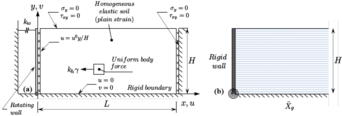
Figure 2.4: Rigid wall with rotating base (a) Wood (1973), (b) Veletsos & Younan (1994b)
