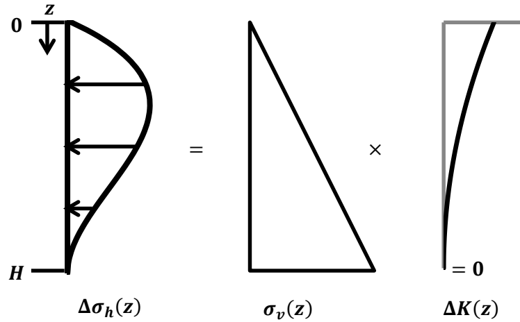
Figure 7.10: Dynamic earth pressure coefficient \Delta K implied by cubic distribution
