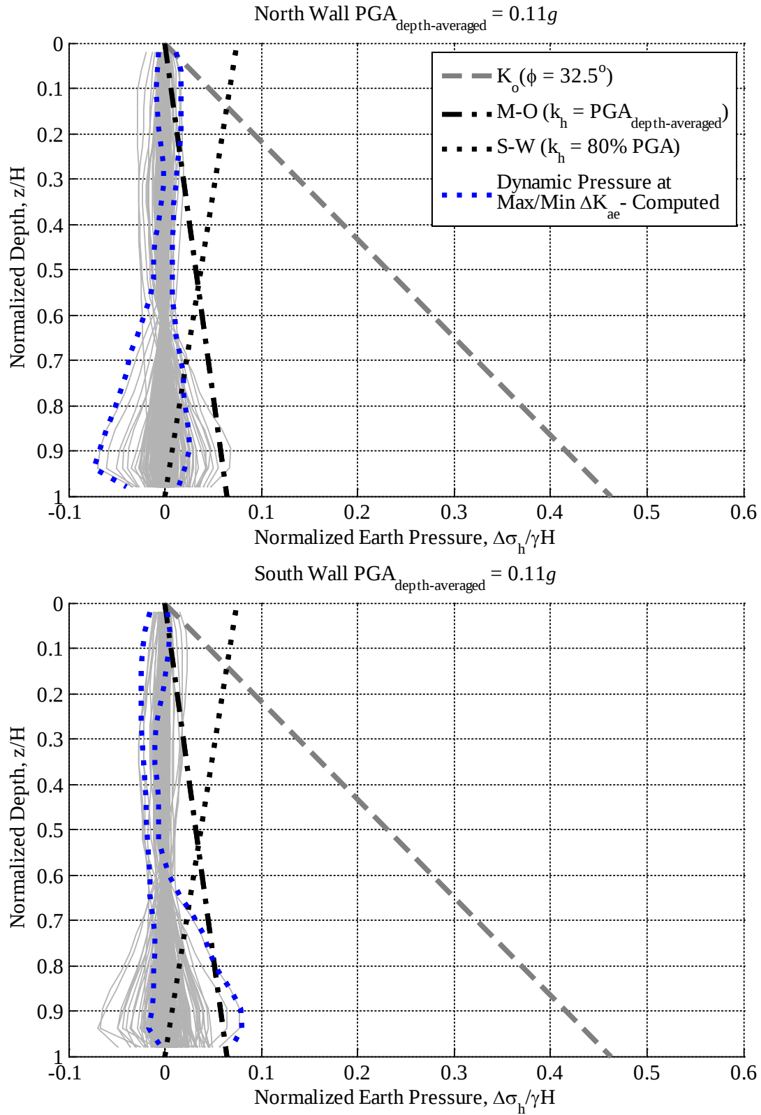
Figure B.44: Computed normalized dynamic earth pressure distributions at maximum and minimum \Delta K_{ae} during Loma Prieta RCH 190 for four level basement; Site Class D
