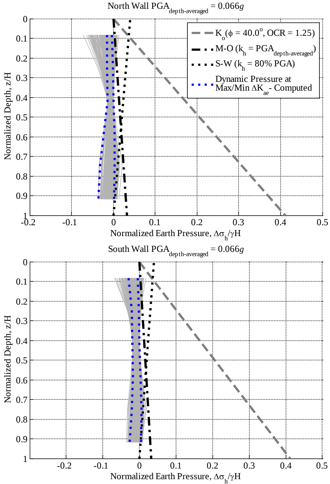
Figure B.122: Computed normalized dynamic earth pressure distributions at maximum and minimum \Delta K_{ae} during Northridge PHP 090 for one bay, one level basement; Site Class C
