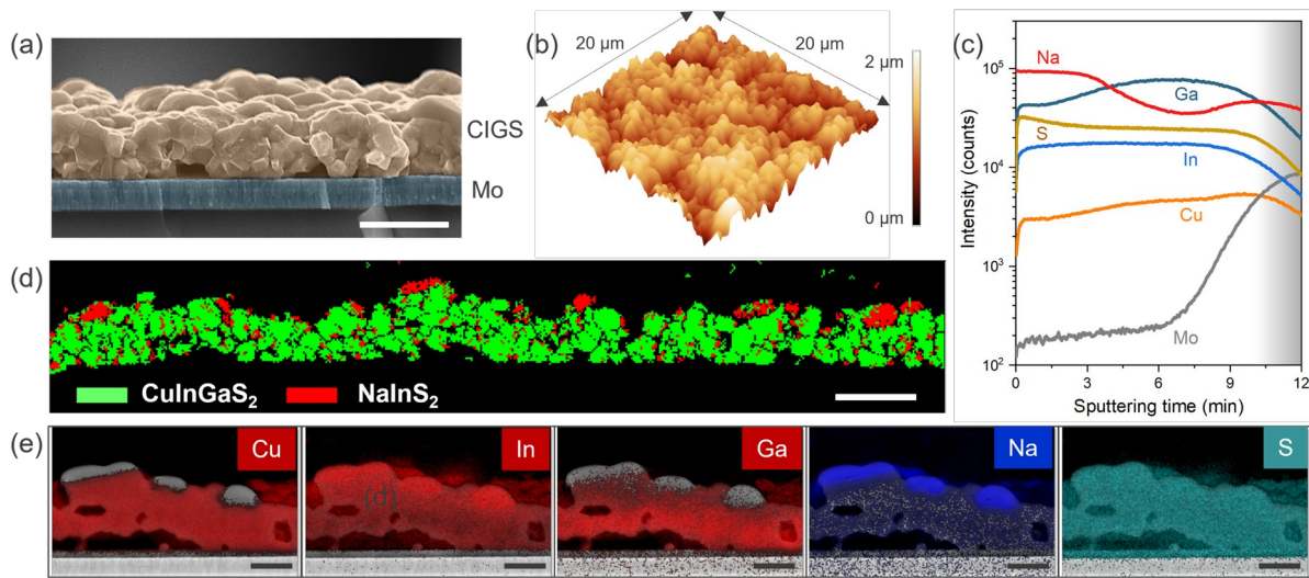
Figure 2. (a) Cross-section SEM micrograph, Scale bar: 2 \mu\text{m} , (b) AFM surface morphology 3D view, and (c) Elemental depth profiles (Cu, In, Ga, S, Na, and Mo) from SIMS analysis of Mo coated
