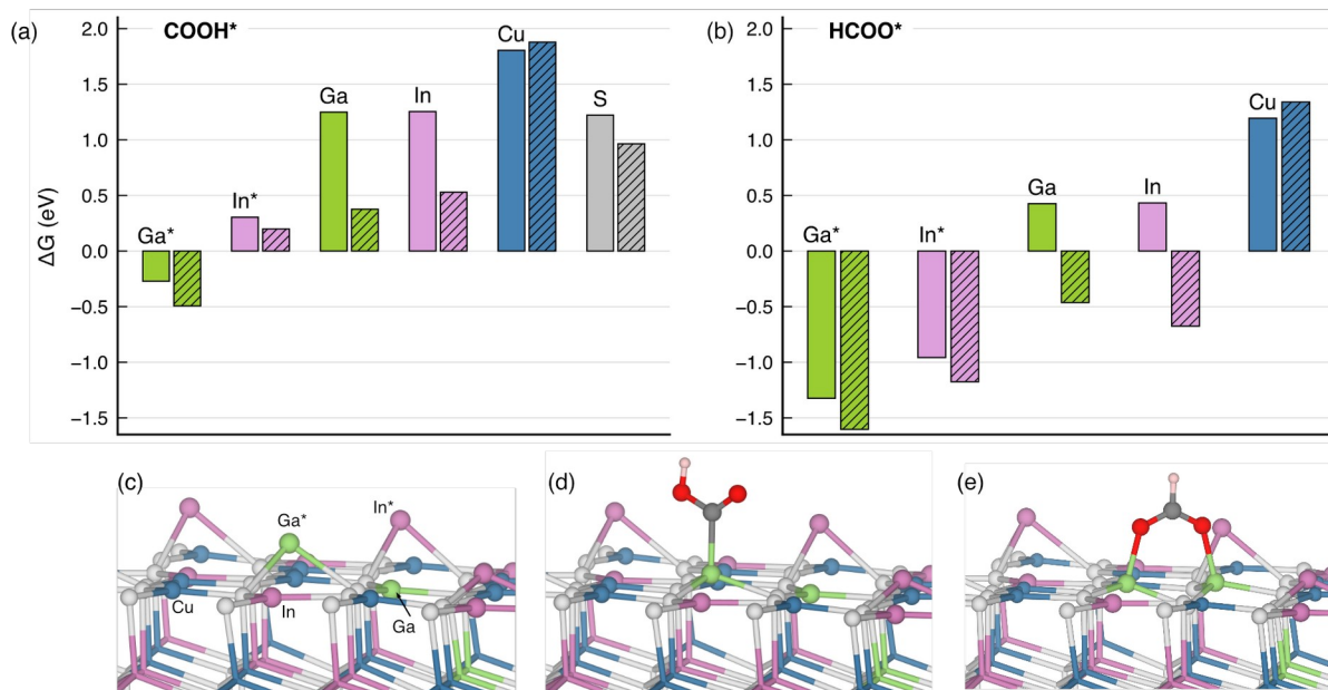
Figure 6. Gibbs free energy of change for the adsorption of (a) \text{COOH}^* and (b) \text{HCOO}^* intermediates on the pristine (solid bar) and the Cu-deficient CIGS (112) surface (shaded bar). The free energies are assessed at room temperature. The adsorption on Cu-deficient CIGS surface occurs at the sites in the close vicinity of a surface Cu vacancy. (c) illustrates the atomic structure of the Cu-deficient CIGS (112) surface prior to adsorption. (d) and (e) correspond to the \text{COOH}^* and \text{HCOO}^* adsorbate structures, respectively.
