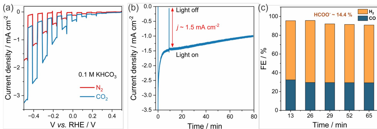
Figure 3. PEC testing of bare CIGS photocathode. (a) Current density vs. potential under 1 sun chopped light measured in \text{N}_2 - and \text{CO}_2 -saturated electrolyte. (b) Current density vs. time at -0.4 V vs RHE for \text{CO}_2 -saturated electrolyte. (c) Time evolution of FE for \text{CO} and \text{H}_2 at -0.4 V vs. RHE. \text{CO}_2 saturated 0.1M \text{KHCO}_3 electrolyte, 1 sun simulated AM1.5G illumination.
