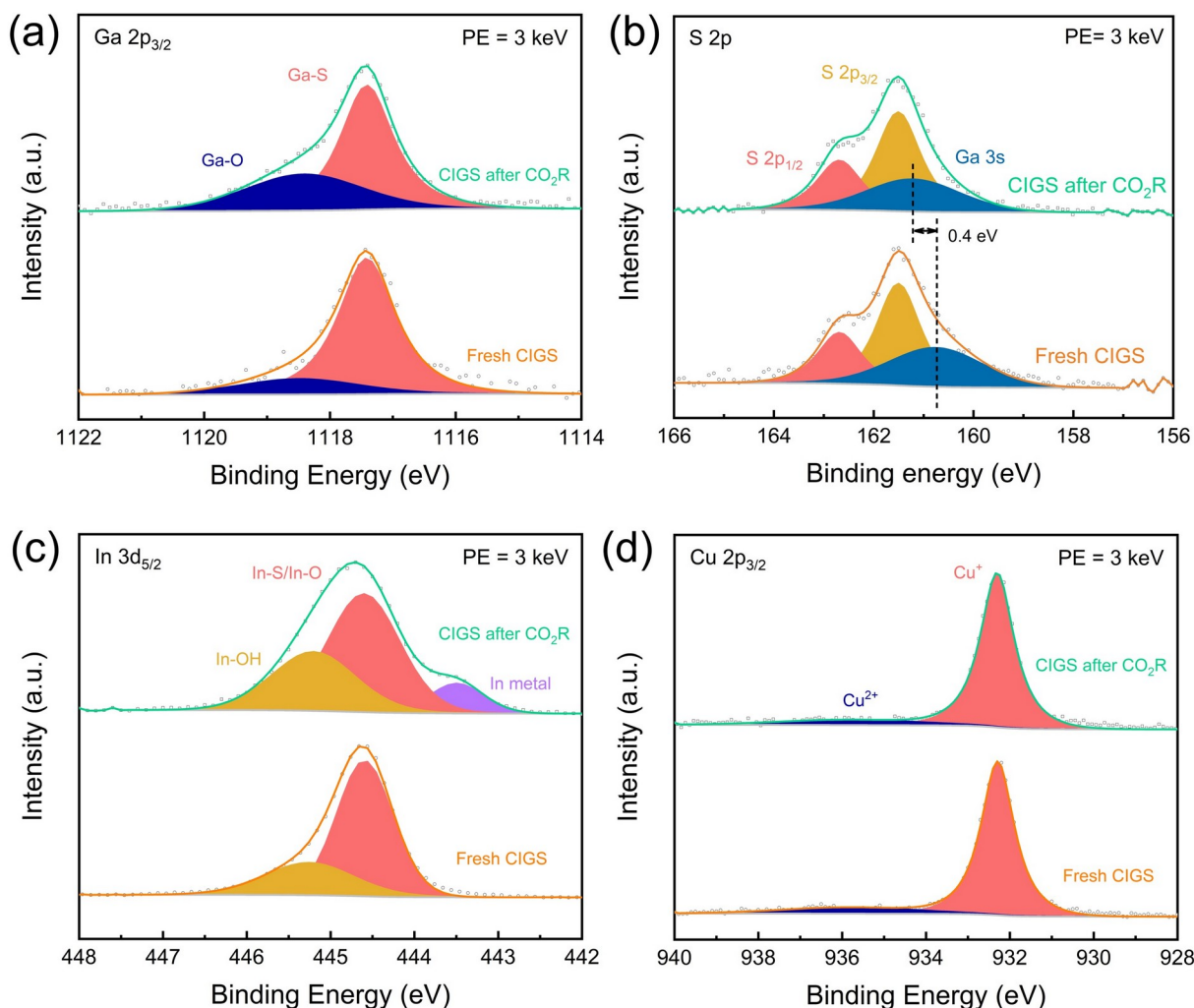
Figure 5. Deconvoluted XPS spectra on the CIGS before and after 80 min of CO 2 R operation. (a) Ga 2p 3/2 , (b) S 2p (c) In 3d 5/2 , and (d) Cu 2p 3/2 photoelectron peaks and curve fitting results (solid color area) of the fresh CIGS (bottom) and CIGS after CO 2 R (upper), respectively (photon energy = 3 keV).
