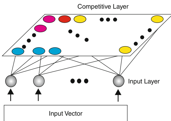
Competitive Learning. Fig. 5 Structure of SOM
