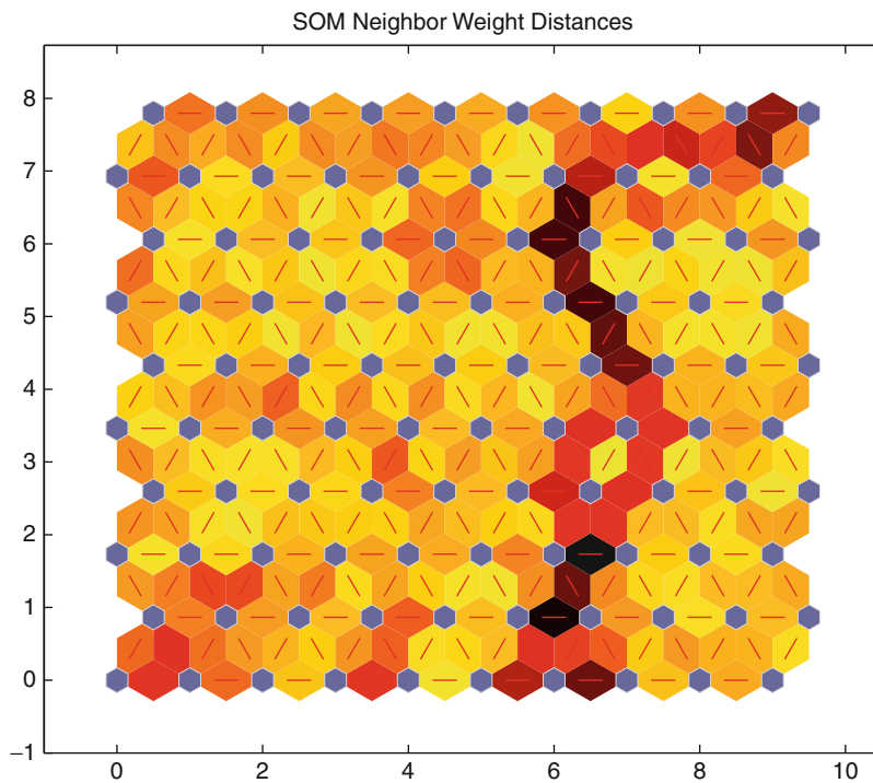
Competitive Learning. Fig. 7 Topological relation
