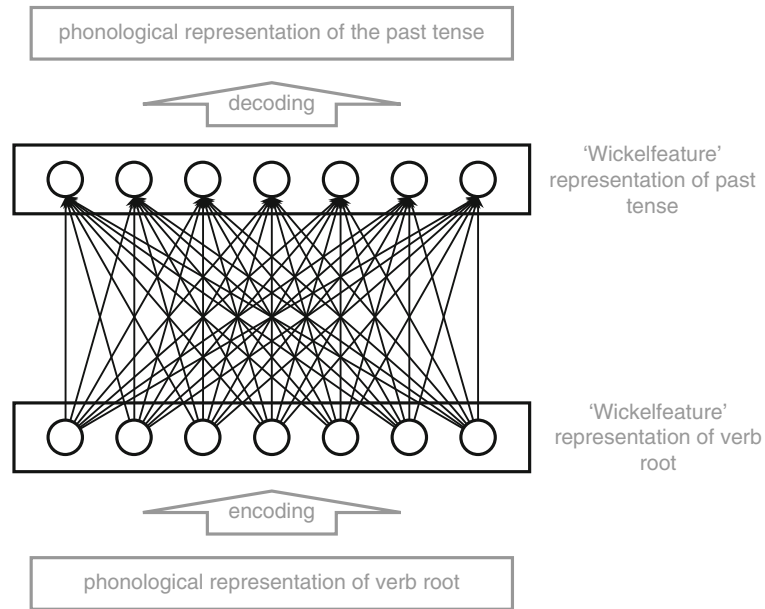
Connectionism. Fig. 3 The Rumelhart and McClelland (1986) model for the learning of the English past tense. The core of the model is a two-layered feed-forward network (pattern associator) which learns mappings between coarse-coded distributed representations (Wickelfeature representations) of verb roots and past tense forms
