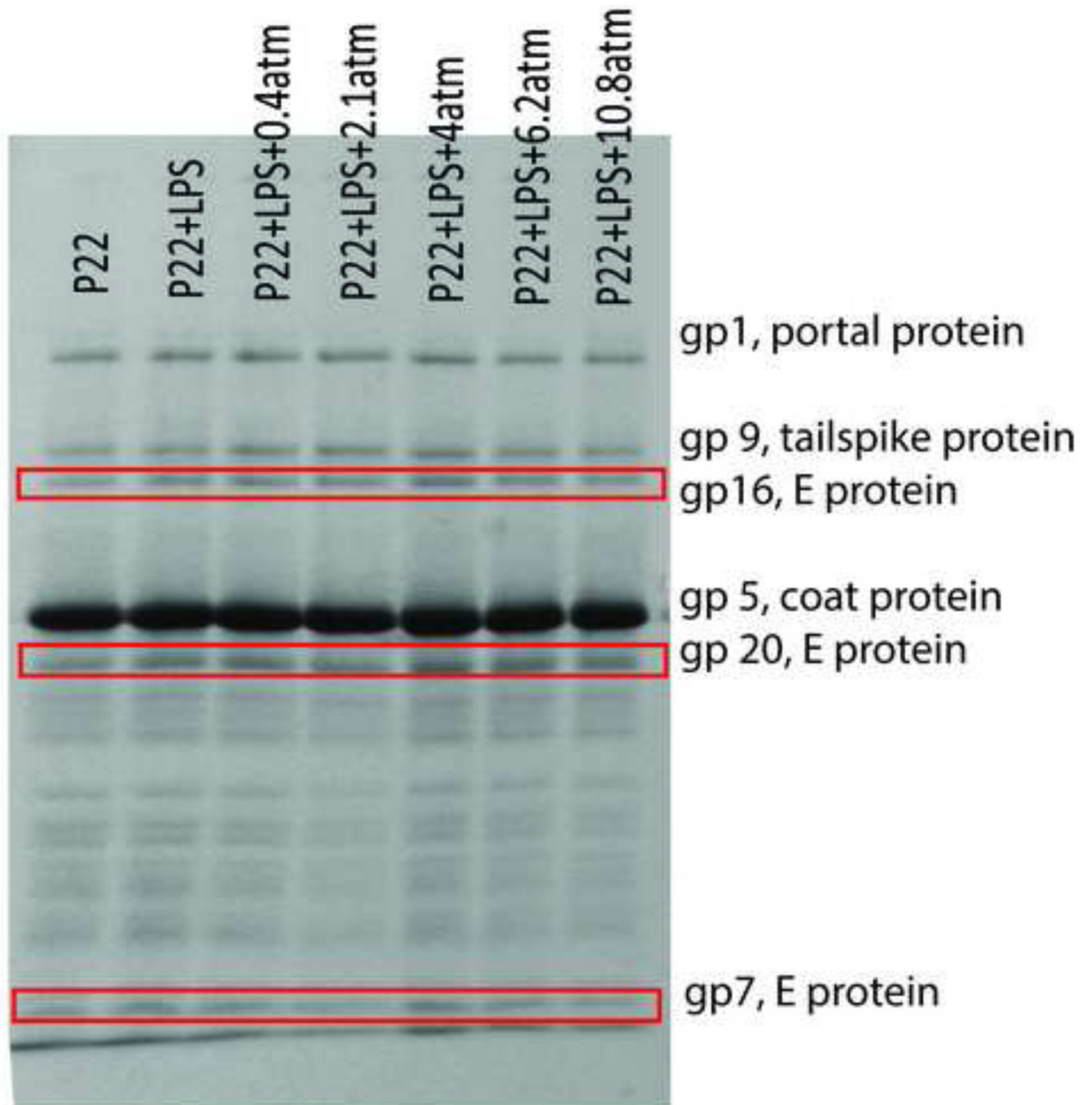
Figure 2. LPS alone is insufficient to eject E proteins
