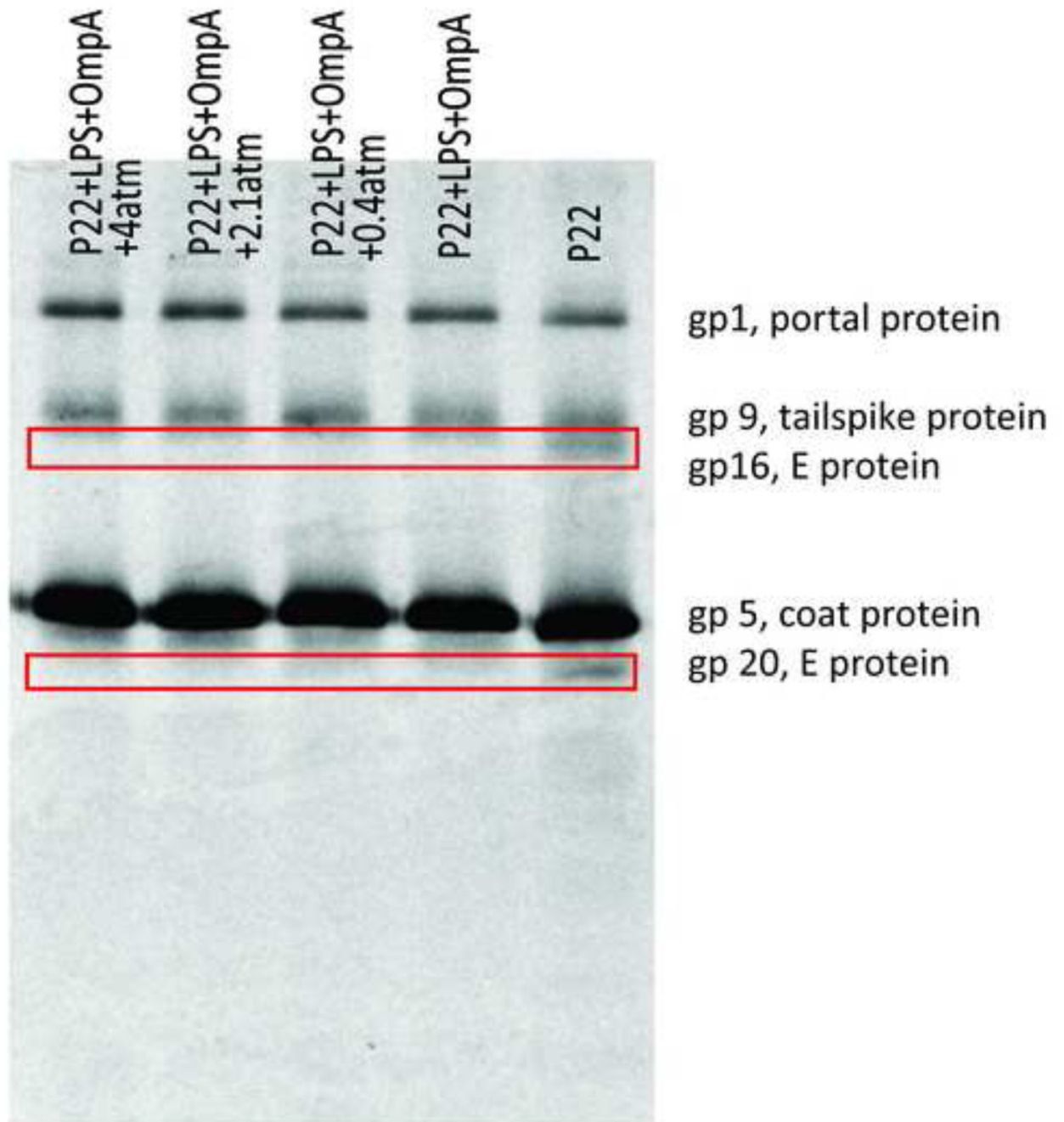
Figure 4. E proteins are ejected in the presence of both LPS and OmpA
