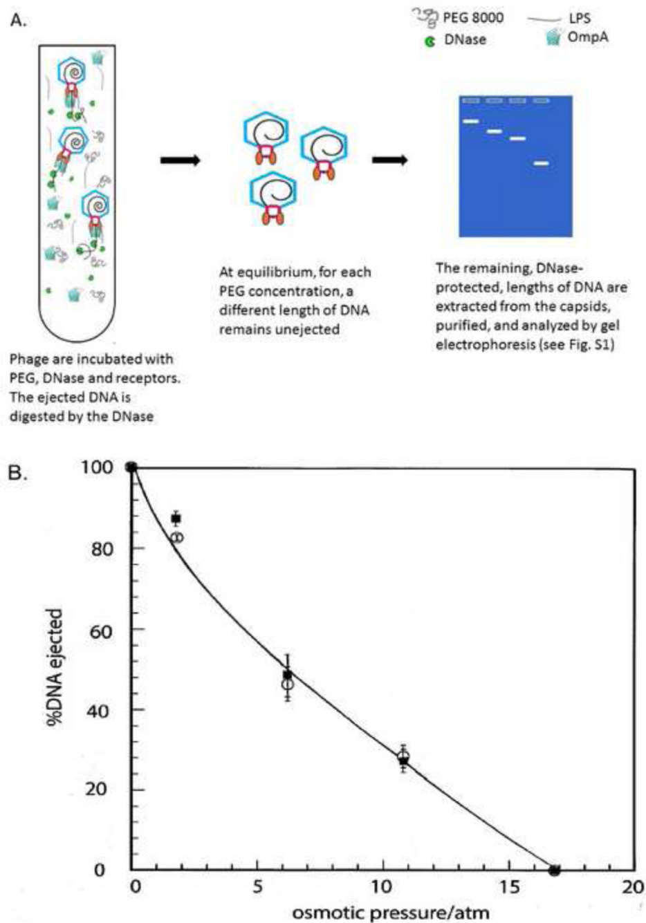
Figure 1. The extent of genome ejection is controlled by osmotic pressure
