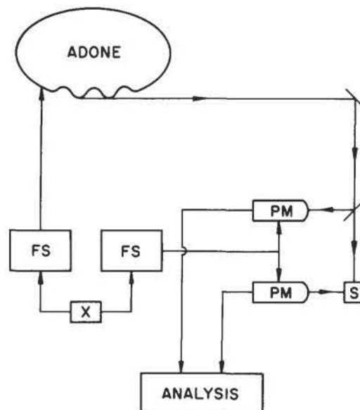
FIG. 4. Block diagram of the instrument. ADONE: storage ring at Frascati; PM: Hamamatsu R928 photomultiplier; S: fluorescence sample; FS: frequency synthesizer; X: crystal oscillator.
