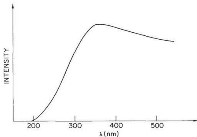
FIG. 3. Spectrum of the incident light passed by the excitation monochromator and detected by the reference photomultiplier.
