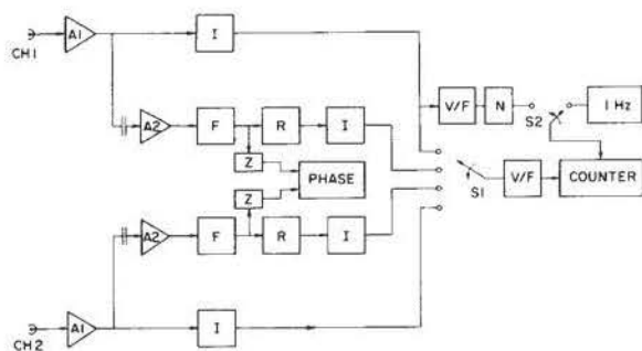
FIG. 6. Block diagram of the electronic detection system. A1, A2: low-frequency amplifiers; I: integrator; F: bandpass filter at 24 Hz; R: rectifier; Z: zero-crossing detector; V/F: 100-kHz voltage-to-frequency converter.
