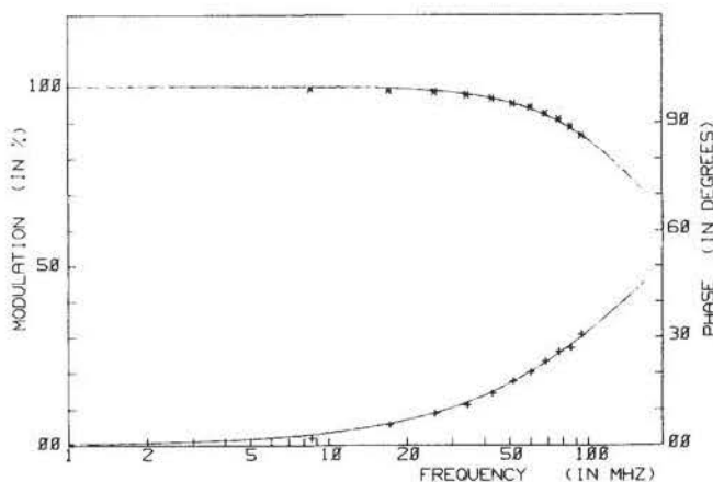
FIG. 7. Multifrequency phase (+) and modulation (*) data for p -terphenyl in cyclohexane at 20°C. Solid lines correspond to the best fit using a single-exponential component \tau_0 = 973 \pm 27 ps.
