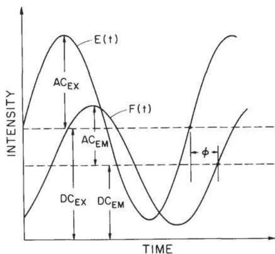
FIG. 1. Schematic representation of the excitation E(t) and fluorescence F(t) waveforms. Fluorescence is delayed by an angle \phi and demodulated with respect to the excitation.
