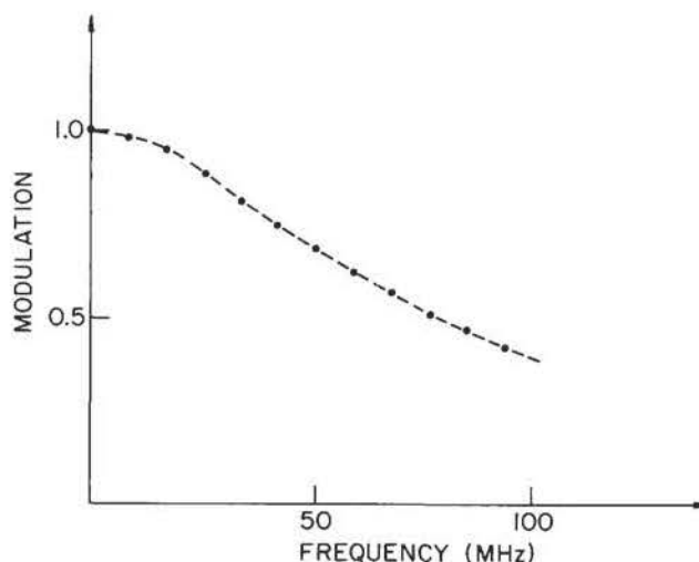
FIG. 5. Relative modulation measured at harmonic frequencies below 100 MHz.
