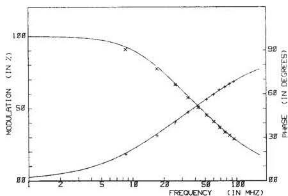
FIG. 10. Multifrequency phase (+) and modulation (x) data for tryptophan at 20°C pH = 9.25. Solid lines correspond to the best fit using two exponential components: \tau_1 = 3.193 \pm 0.026 ns, \tau_2 = 9.00 ns, and f_1 = 0.396 \pm 0.005 .
