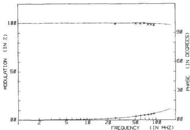
FIG. 8. Multifrequency phase (+) and modulation (x) data for bis -ANS in water at 20°C. Solid lines correspond to the best fit using a single-exponential component \tau_0 = 196 \pm 10 ps.
