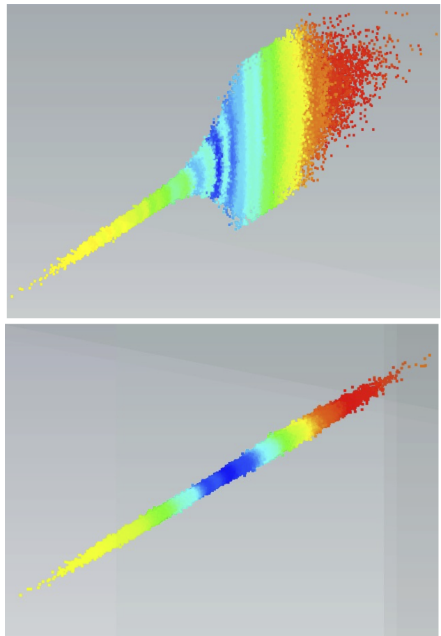
Figure 4: Top: final transverse spatial distribution after propagation in simple slab from CST simulation, displaying quadrupole instability. Bottom: final distribution after traversal of alternating symmetry structure, showing strong focusing.
