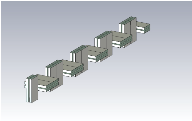
Figure 3: Simple slab DWA with structures rotated 90 degrees periodically to obtain second order quadrupole focusing.
