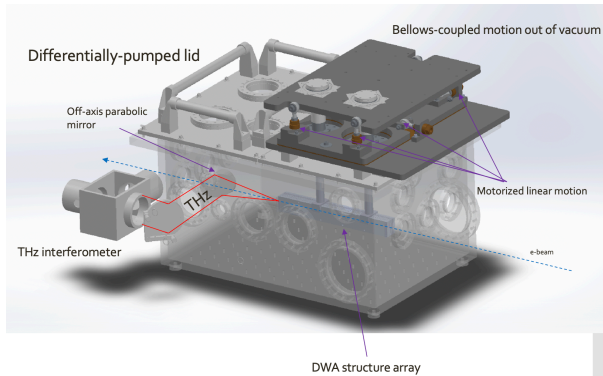
Figure 1: Rendering of vacuum vessel design for hosting DWA experiments at FACET-II.
