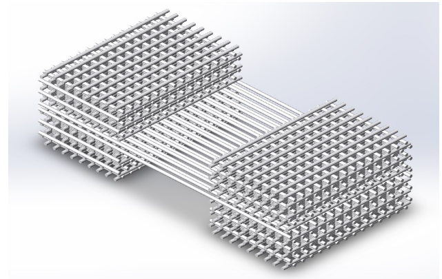
Figure 2: Optimized hybrid woodpile photonic structure for DWA experiments, permitting mode control and HOM damping.
