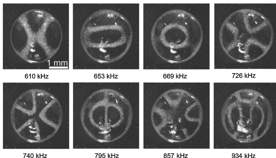
FIG. 24. As the excitation frequency is raised, distinct patterns appear as defined by the pinning of the particles within a sessile drop; the drop is \sim 2 mm in diameter and 1 mm in height. From Oberti, Neild et al. , 2009.
