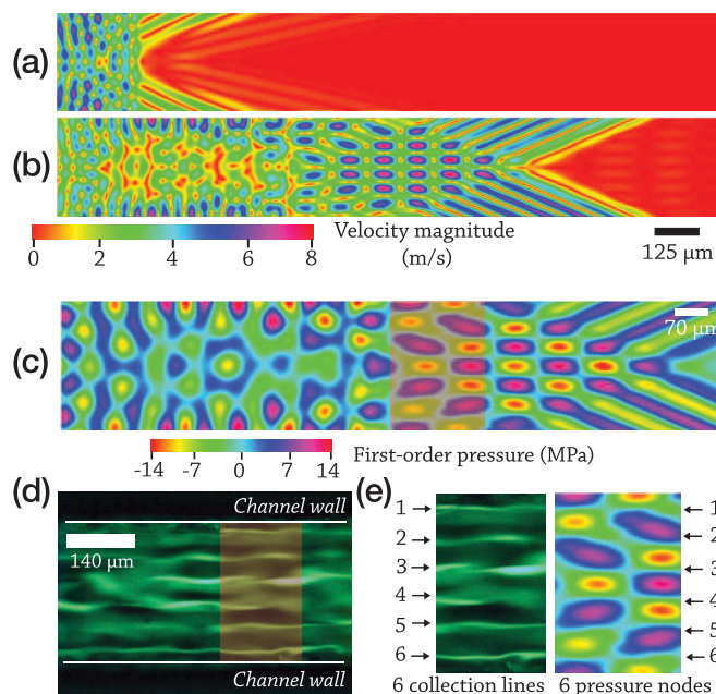
FIG. 27 (color online). The magnitude of the fluid velocity in a 280 \mu\text{m} wide channel (see Fig. 13) viewed from the top down with x_1 from left to right, due to 20 MHz acoustic waves refracting into the water in the channel from the LN after (a) 4 and (b) 10 cycles of the SAW. This model incorporates bidirectional coupling between the piezoelectric LN and the fluid, and (c) the cross-channel standing wave with its pressure nodal lines causes (d) particles to collect along six distinct lines across the width of the channel, directly corresponding (e) to the pressure node lines. From Tan, Yeo, and Friend, 2009.
