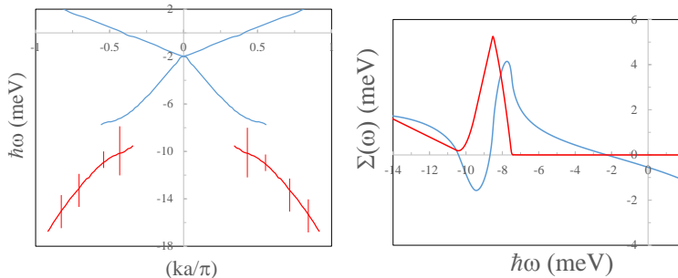
Figure 3: The calculated quasi-particle T = 0 dispersion relations along the diagonal line (k, k) of the two-dimensional surface Brillouin zone (Left) and the frequency-dependence of the T = 0 self energy \Sigma(\omega) (Right). The real part of the self energy is shown in blue and the imaginary part is shown in red. (Colour online)
