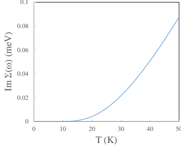
Figure 2: The thermally activated temperature dependence of the imaginary part of the self energy due to interactions with spin-excitons, for electrons on the surface Fermi-surface. (Colour online)
