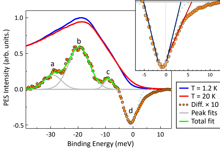
Figure 1: The angle integrated valence-band photoemission spectra measured at the sample temperatures of 1.2 K (blue line) and 20 K (red line). The difference between the spectra at these two temperatures is shown in orange. To enhance the excursions, the difference spectrum has been multiplied by a factor of 10. The inset shows a close up of the difference spectrum near the Fermi-energy. Spectra were measured along the \bar{X} - \bar{\Gamma} - \bar{X} direction in the BZ and integrated over the entire angular range of the detector (30 deg). (Colour online)
