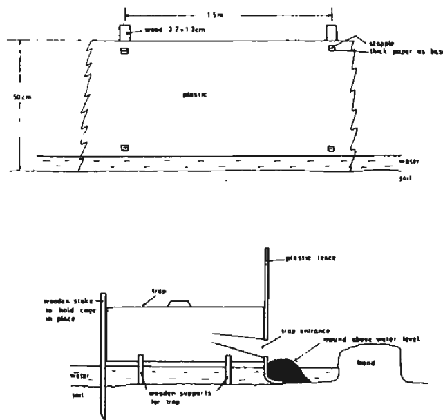
Fig. 2. Design and construction of the plastic fence and the placement of the trapping device.
