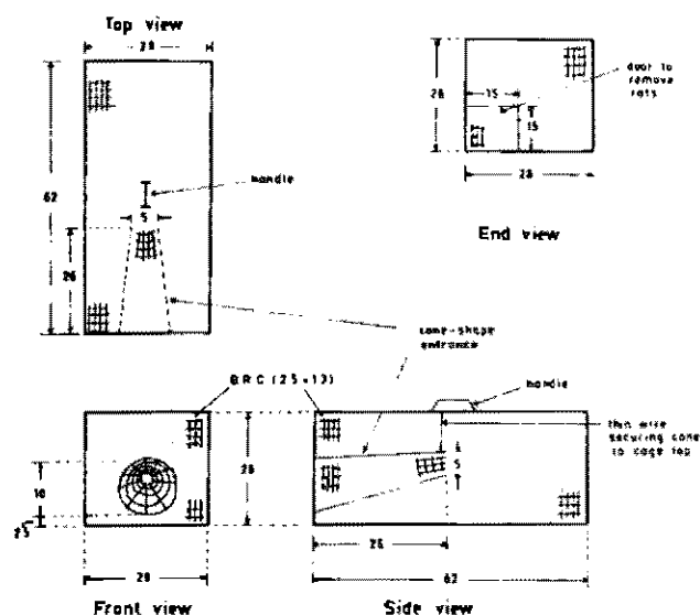
Fig. 3. Design of the trap (All measurements are in centimeters).
