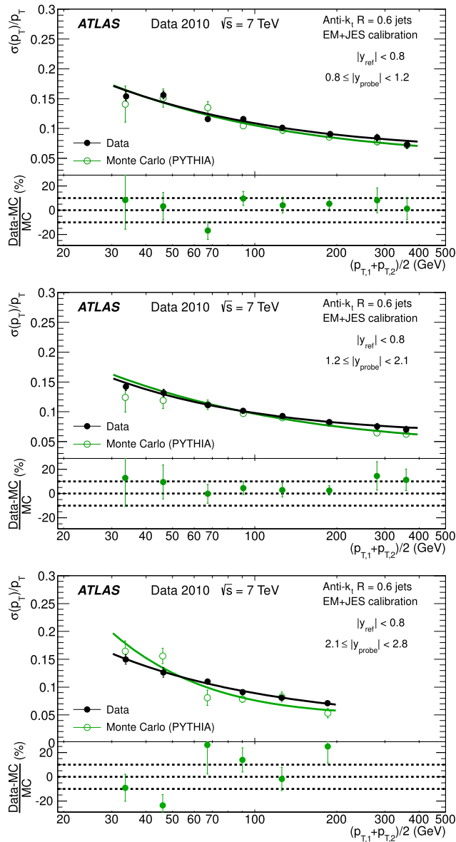
Fig. 9 Fractional jet p_T resolution as a function of \bar{p}_T for anti- k_r with R = 0.6 jets in the Extended Tile Barrel ( top ), Transition ( center ) and End-Cap ( bottom ) regions using the bisector method. In the lower panel of each figure, the relative difference between the data and the MC simulation results is shown. The dotted lines indicate a relative difference of \pm 10\% . The curves correspond to fits with the functional form in Eq. (9). The errors shown are only statistical
