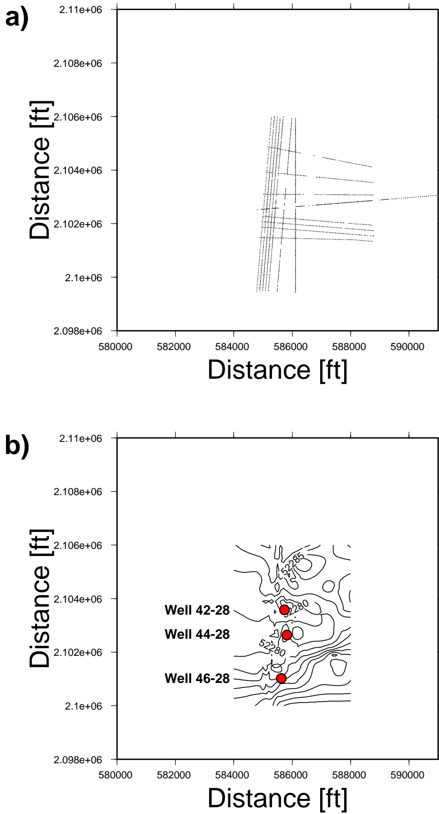
Figure 14. Results of gravity measurements at Rye Patch within the boundaries of the 3-D seismic survey area. a) Location of gravity measurements. b) Contour map of Bouguer gravity residual.
