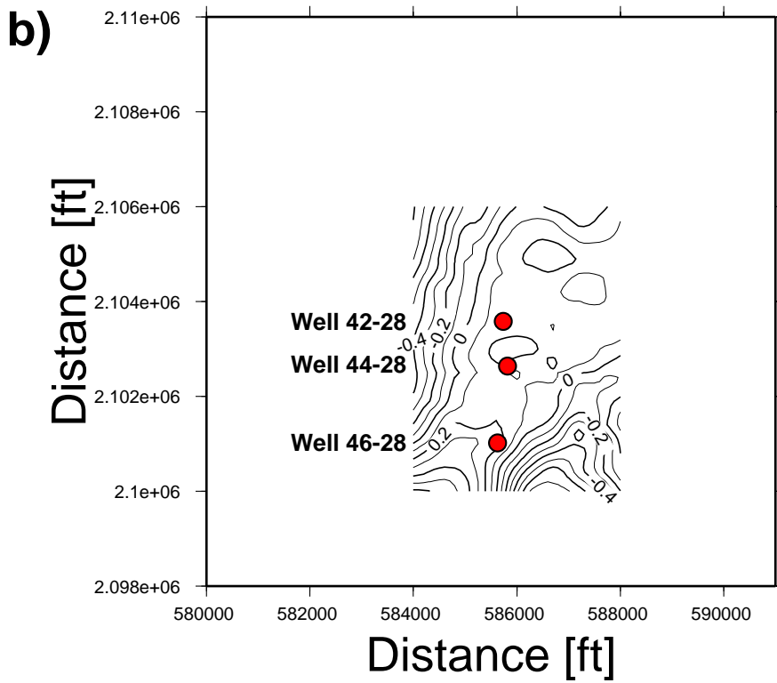
Figure 15. Results of magnetic measurements at Rye Patch within the boundaries of the 3-D seismic survey area. a) Location of magnetic measurements. b) Contour map of total magnetic field.
