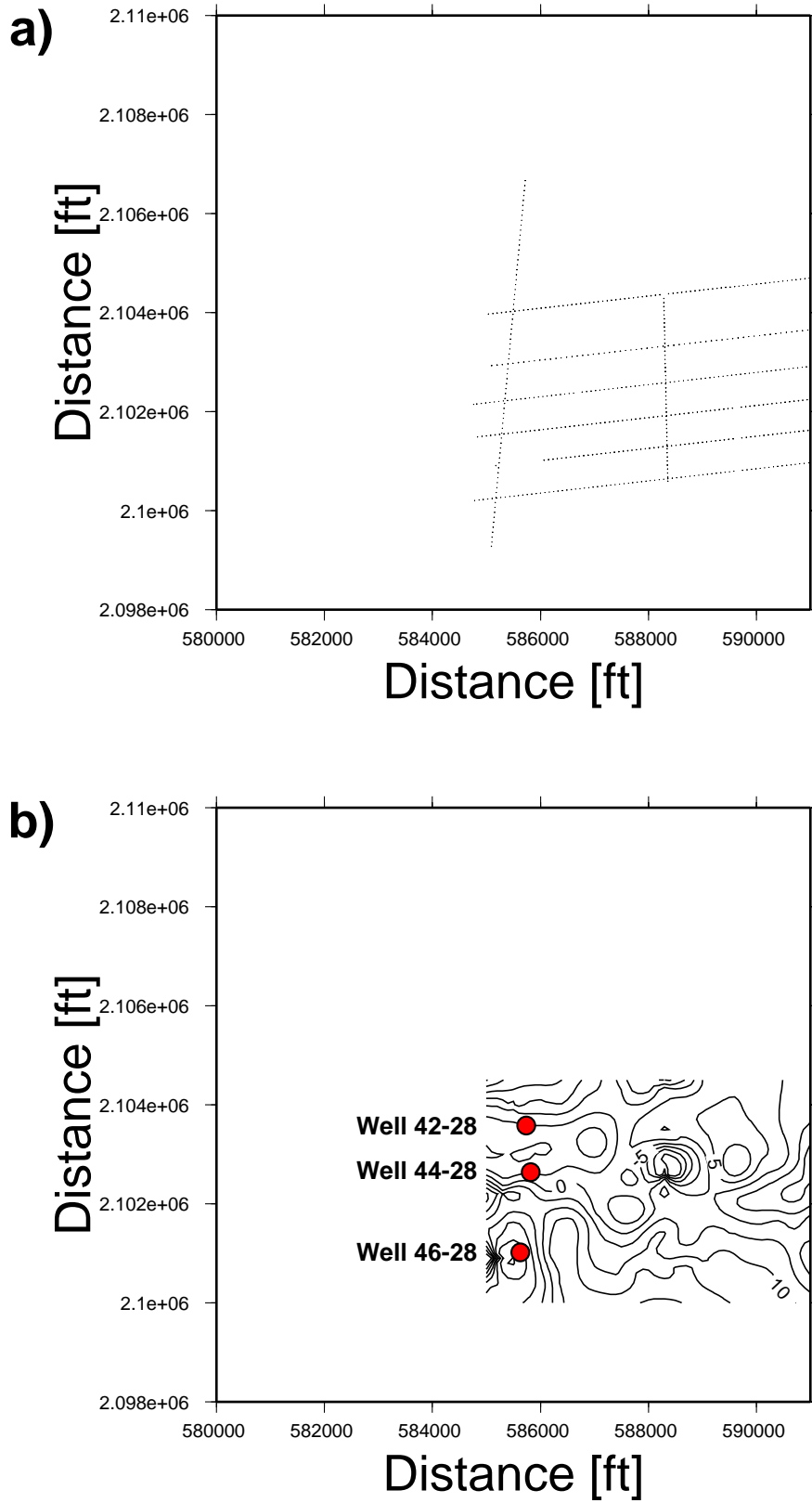
Figure 16. Results of self potential measurements at Rye Patch within the boundaries of the 3-D seismic survey area. a) Location of self potential measurements. b) Contour map of self potential field.
