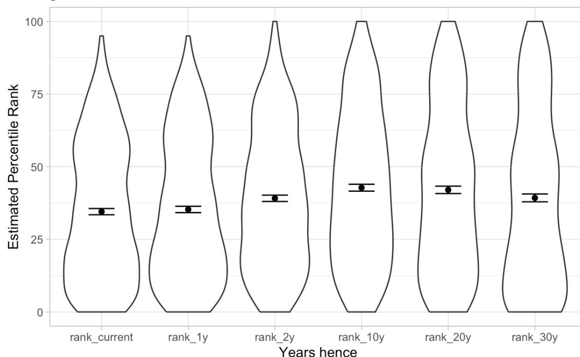
Figure 2. Respondents underplace their incomes, as shown in this violin plot of respondents' estimates of their rankings in the income distribution at six points in time ( n=490 ). The width of each white blob indicates the density of responses at each level. Black dots indicate means, with error bars indicating one standard error above and below the sample mean.
