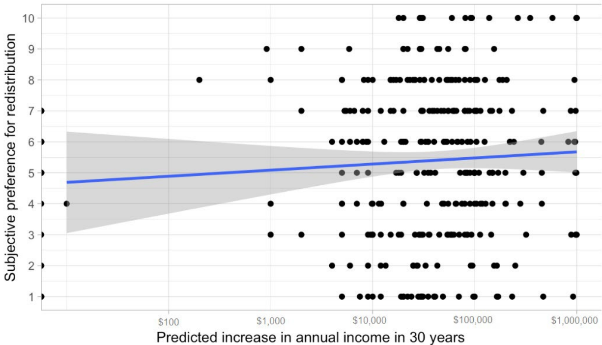
Figure 3. No evidence of the POUM hypothesis in a scatterplot of predicted increase in income 30 years hence (log scale) and subjective support for redistribution in response to the question, “How much redistribution do you want among citizens?” on a scale from 1: No redistribution, to 10: Complete redistribution, for the full sample ( n=490 ).
