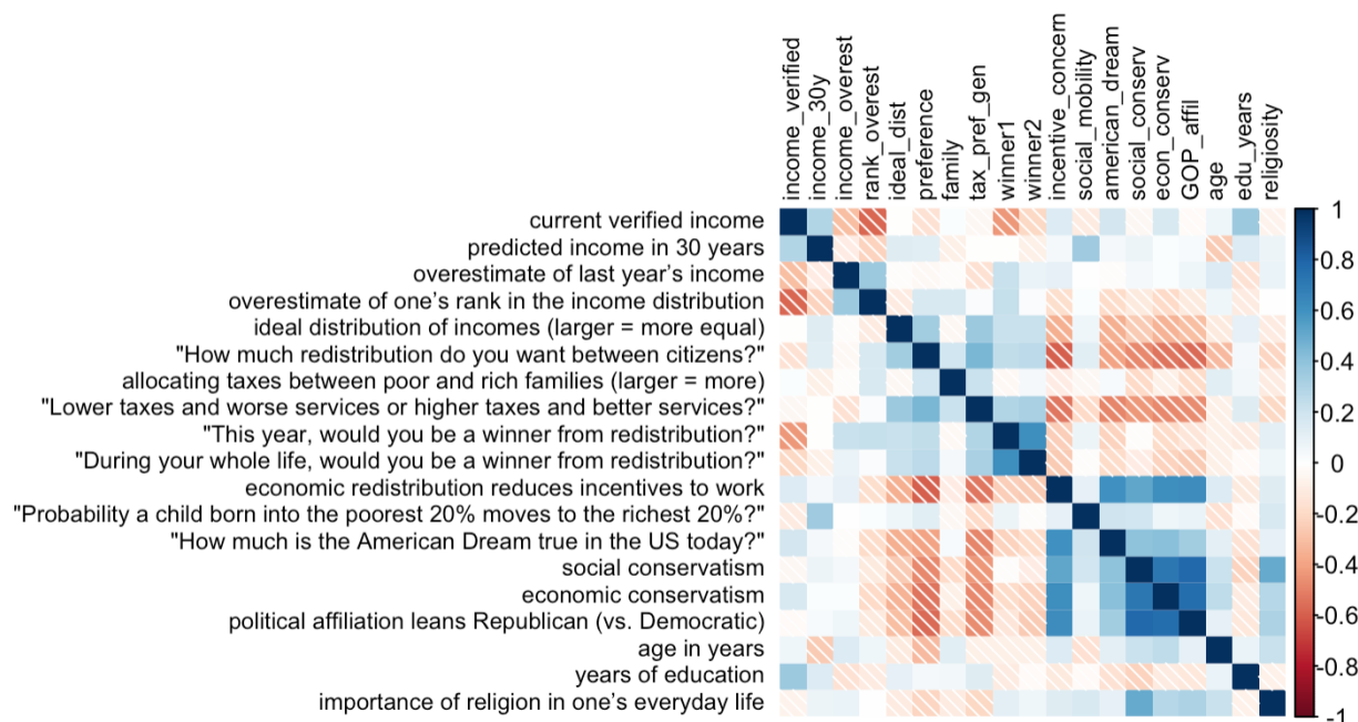
Figure 1. Predicted future income is weakly associated with attitudes toward redistribution in a correlation matrix showing associations between measures ( N=134 ), with variable names along the top and descriptions on the left. Darker blue squares indicate stronger positive correlations; darker red cross hatched squares indicate stronger negative correlations; white squares indicate faint or zero-order correlations.
