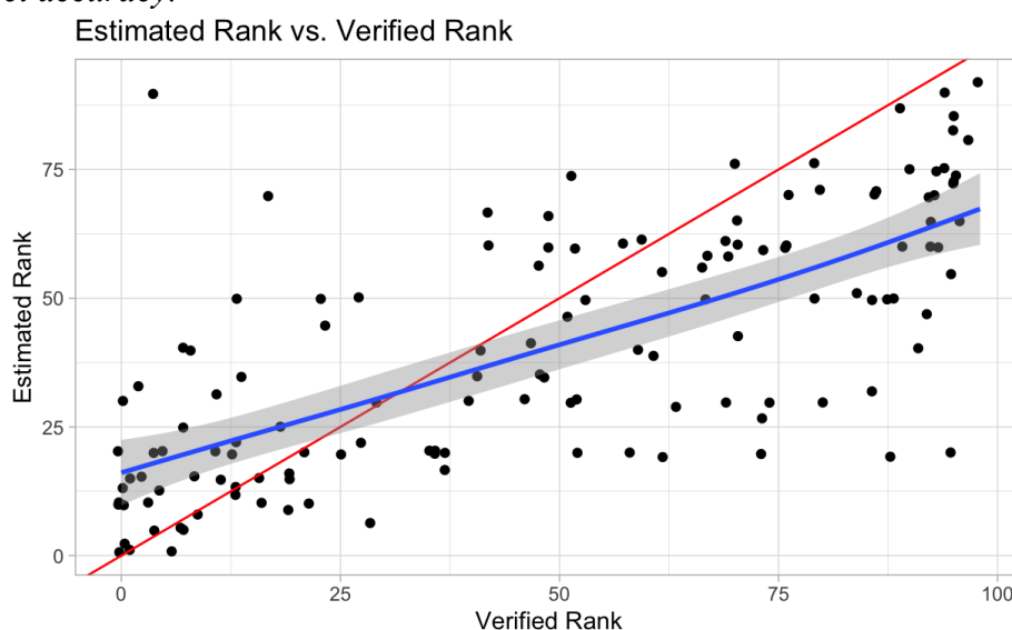
Figure 4. Scatterplot of estimated vs. verified percentile rank shows the “middle class” effect. Data from those who verified their income ( n=135 ). The red identity line represents perfect accuracy.
