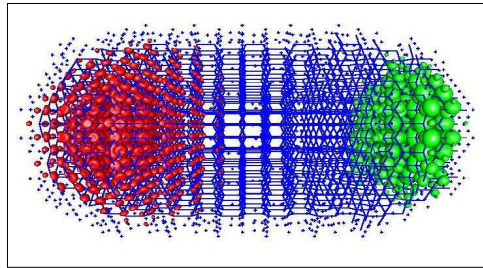
FIG. 4: The electron (red) and hole (green) states shown in their isosurfaces with an isovalue of 0.0002 \text{ e/Bohr}^3 in the \text{Cd}_{961}\text{Se}_{724} wurtzite structure quantum rods with Cd atom terminations.
