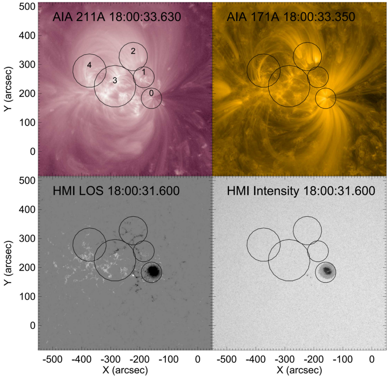
Fig. 3. Regions analyzed overlaid on SDO images. Top row: two AIA filters that have sensitivity to quiescent coronal temperatures, and bottom row: HMI line-of-sight magnetogram and intensity map. Images shown are at a time near the middle of the analyzed interval. At the latitude of this active region, solar rotation causes sources to drift westward at a rate of about 10 arcsec per hour.
