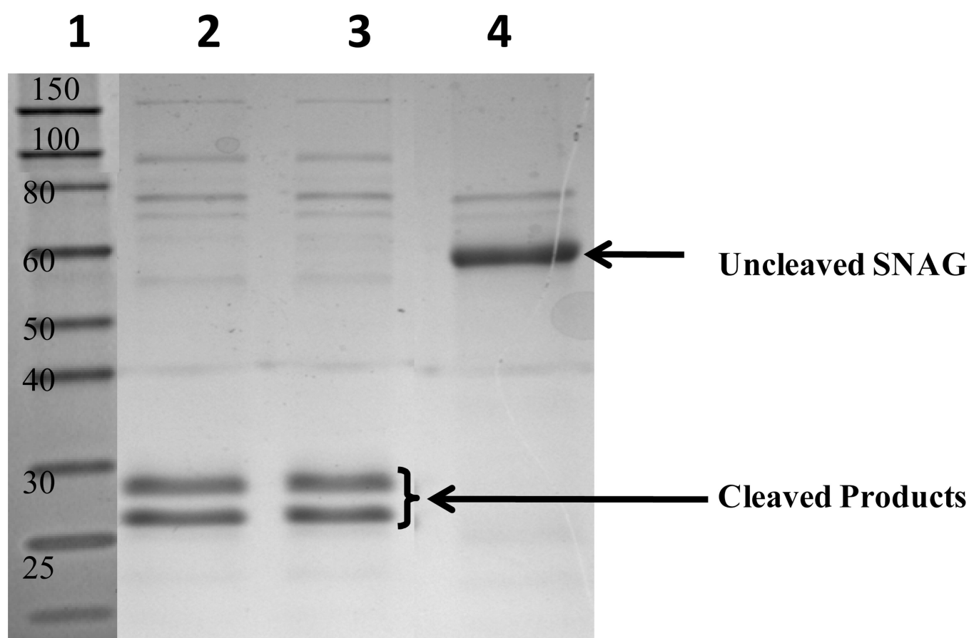
Figure 7. SNAG-Endopeptidase assay demonstrating no effect of low pH elution on enzymatic activity of BoNT/A. Lane 1 – Broad range molecular weight marker, Lane 2 and 3 – Endopeptidase cleavage products of SNAG by non-treated (control) BoNT/A and BoNT/A neutralized after pH 2.5 treatment, respectively, Lane 4 – Uncleaved SNAG protein control.
