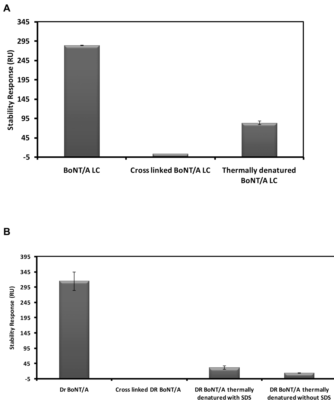
Figure 3. Specific recognition of natively folded, active BoNT/A LC (A) and DR BoNT/A (B) by S132B-C22 aptasensor. Data showed are the average of two independent measurements, with error bar as the standard deviation.
