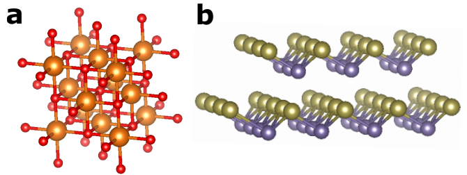
FIG. 2. Structures of MgO (panel a) and GeTe (panel b). Mg atoms are shown in orange, O in red, Ge in purple, and Te in gold. The structures are visualized in VESTA [74].
