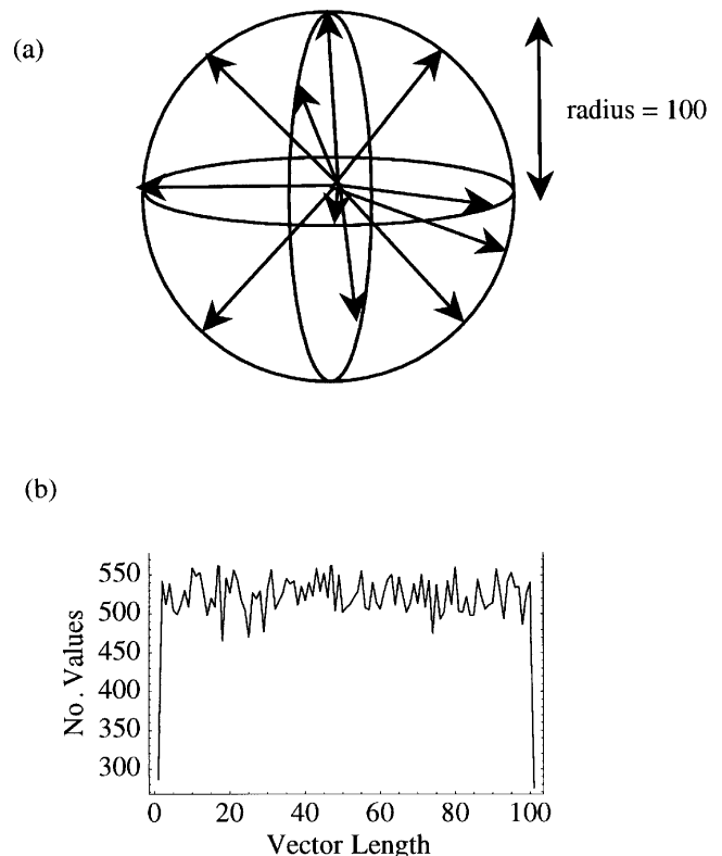
Fig. 5. Simulation illustrating the relationship between a set of 50 000 three-dimensional translations and the actual one-dimensional projections that are measured by the system. (a) The three-dimensional translations are all of the same magnitude, x' , however isotropically oriented. (b) Values that would be measured by projecting this set of three-dimensional vectors onto a single one-dimensional vector, corresponding to the actual range measurements that the sonar would be making.
