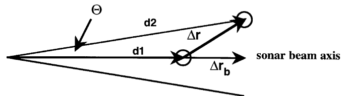
Fig. A1. Geometric projection of the true three-dimensional displacement onto the range axis of the sonar beam.
