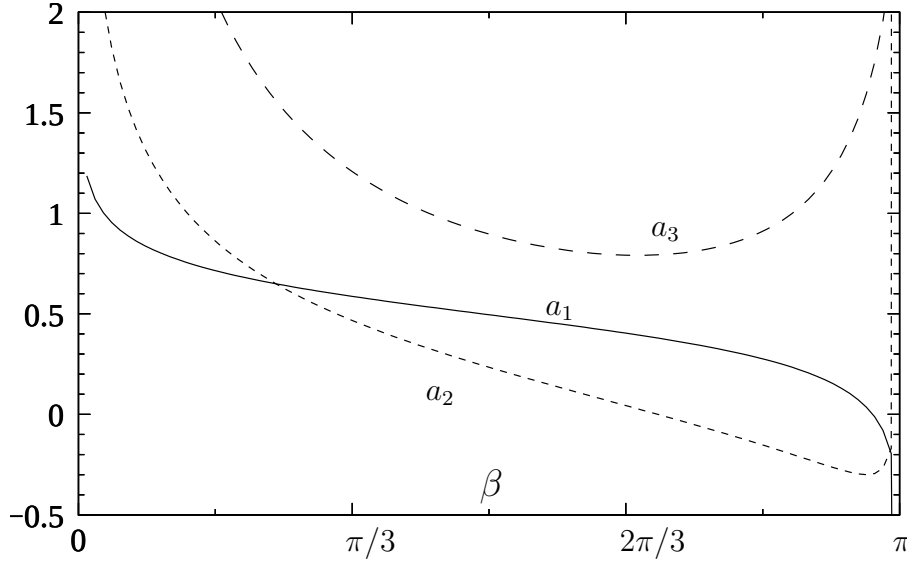
FIGURE 8. Coefficients a_k as functions of \beta as given by (7.18) and 7.9).
