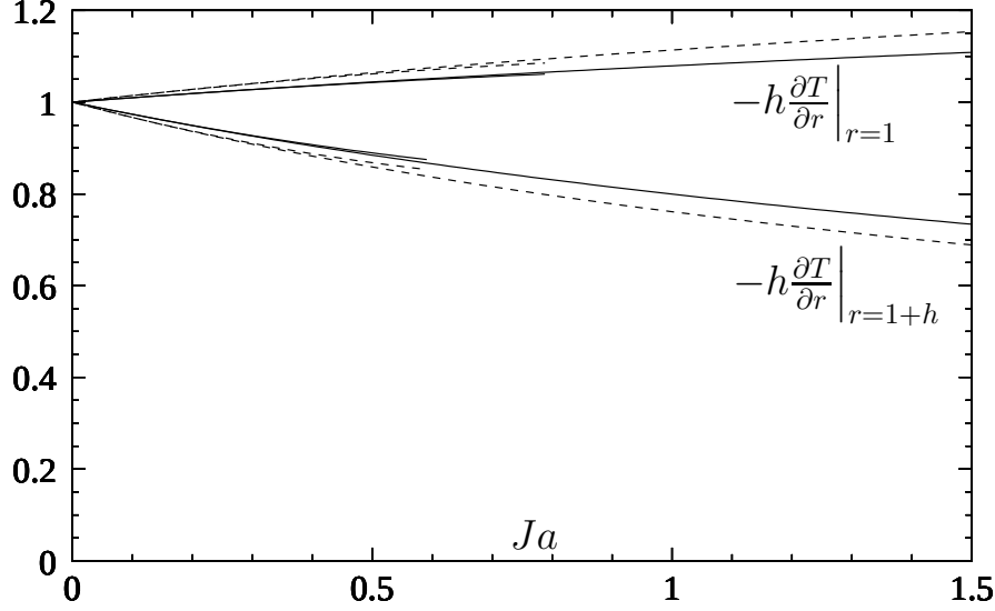
FIGURE 2. Product of film thickness and heat flux as given by the similarity solution (B7). Solid and broken curves show the effect of the boundary condition on v_\theta at the vapour side of the interface: solid curves, \partial v_\theta / \partial r = 0 ( c = 3 ); broken curves; v_\theta = 0 ( c = 12 ). Short curves, Taylor series (B9) to O(Ja^2) .
