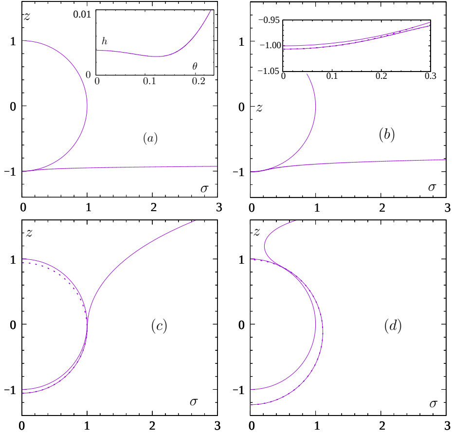
FIGURE 4. Interface profiles for JaCr = 10^{-8} and values of p_0 at, or to the right of, the maximum in figure 3a: (a) p_0 = 2.4311 ( F/(JaCr)^{1/3} = 10.24 ), inset showing the local minimum in h ; (b) p_0 = 2.35 ( F/(JaCr)^{1/3} = 28.78 ), inset showing the spherical cap used to determine the contact angle \chi ; (c) p_0 = 2.0 ( F/(JaCr)^{1/3} = 464.1 ); and (d) p_0 = 1.8 . Solid curves, numerical solution of (3.3). Broken curves, sphere osculating with the interface at its lowest point.
