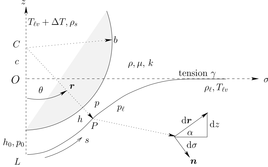
FIGURE 1. Cylindrical coordinates (\sigma, z) , z = 0 on the flat interface. Sphere: centre C at z = c . Liquid–vapour interface: s = |LP| , arc length from the lowest point L to point P ; \mathbf{r}(s) = CP , position vector of point P . Vapour layer: thickness h = |\mathbf{r}| - b , pressure p ; h_0, p_0 , values at s = \theta = 0 . Inset: unit normal \mathbf{n} ; tangent d\mathbf{r} , inclination \alpha ; ds = |d\mathbf{r}| .
