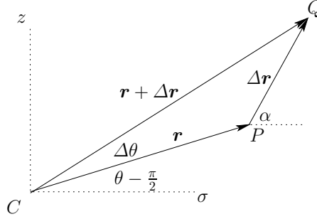
FIGURE 12. Geometry used to prove the identities (3.3d, e): position vectors CP and CQ of two arbitrary points on the interface; \Delta\theta = \angle PCQ is of arbitrary magnitude.
