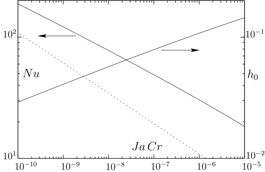
FIGURE 5. Solid lines, values of Nu and h_0 from the numerical solution of (3.3) for p_0 = 2 , approximating the state of maximum force in figure 3. Broken line, (4.3) for the value Bo = 0.03 used for the example. The relative error in the values of Nu is O(Nu^{-1}) .
