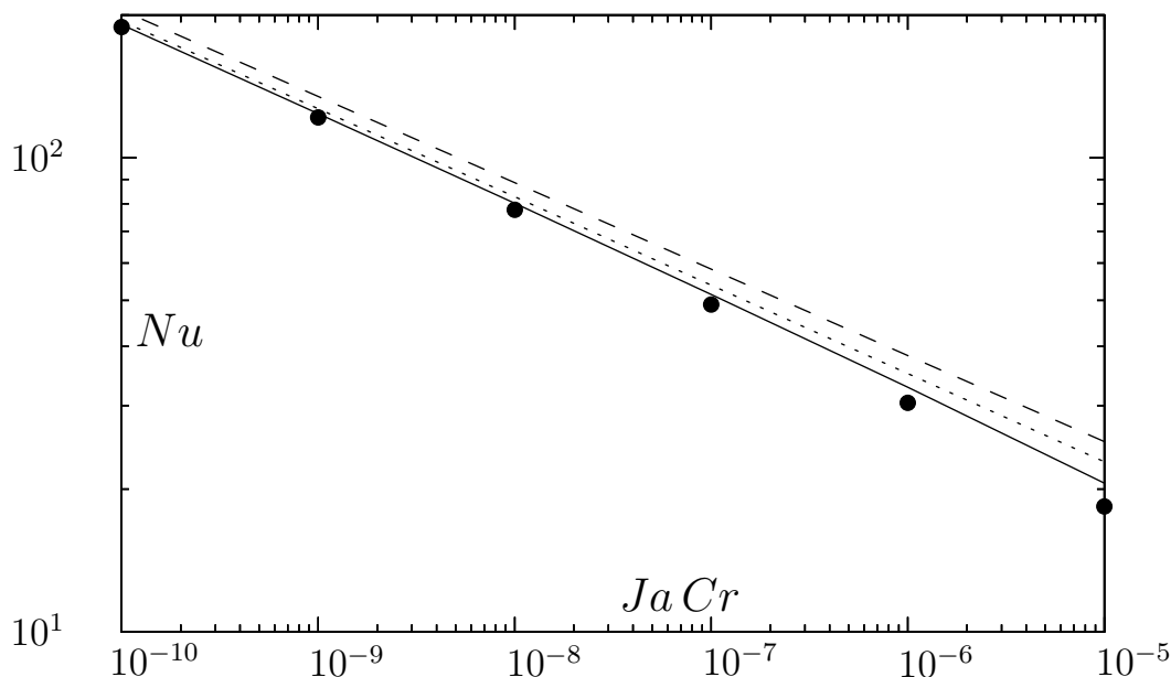
FIGURE 11. Nusselt number for p_0 = 2 as a function of JaCr . Symbols, numerical solution of (4.3). Lines show the effect of truncating the series (8.1) at various orders: O(\lambda) , - - - ; O(\lambda^2) , --- ; O(\lambda^3) , \cdots .
