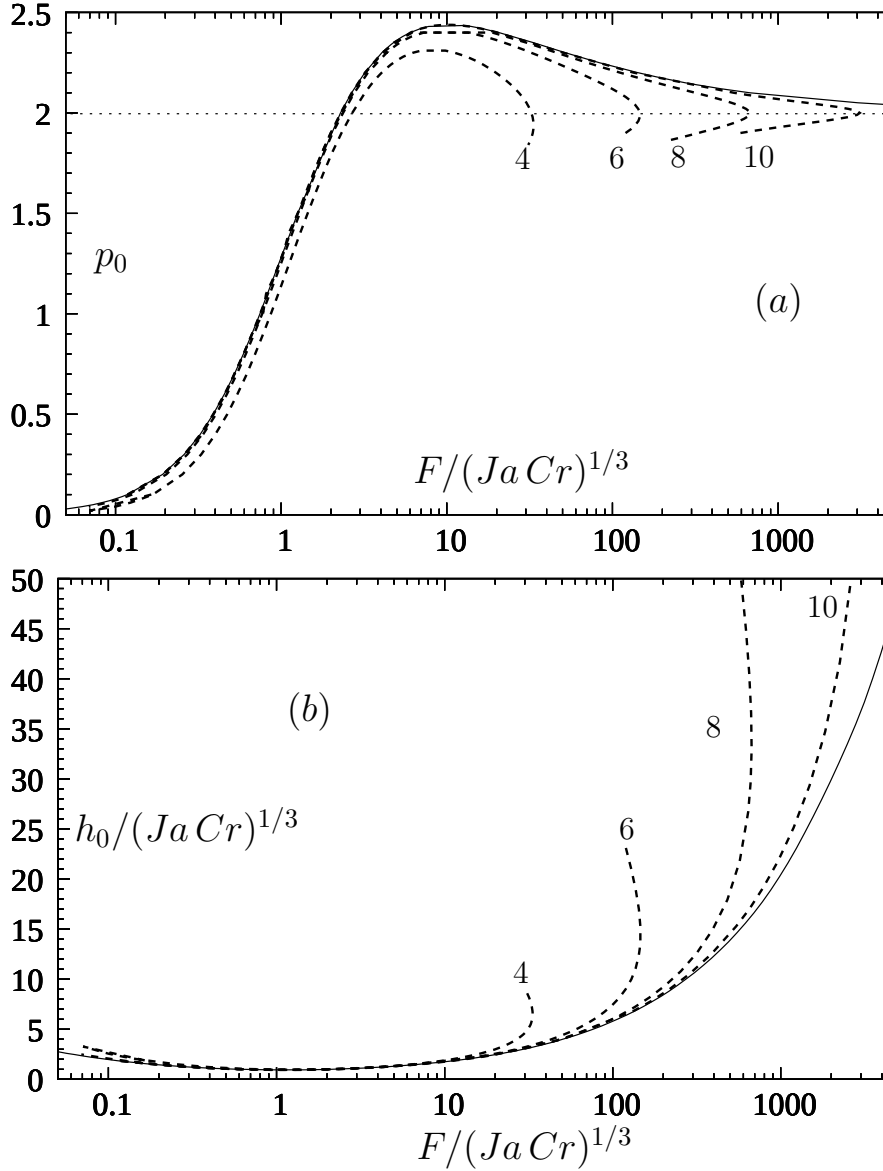
FIGURE 3. Pressure and film thickness at the stagnation point at \theta = 0 . Broken curves, numerical solution of (3.3) for the values of -\log_{10}(JaCr) indicated by the labels. Broken curves have two branches; as indicated by the dotted horizontal line in (a), the branch point occurs asymptotically at p_0 = 2 . Solid curve, solution of the simplified system (E2) describing the limit JaCr \rightarrow 0 (fixed F/(JaCr)^{1/3} ).
