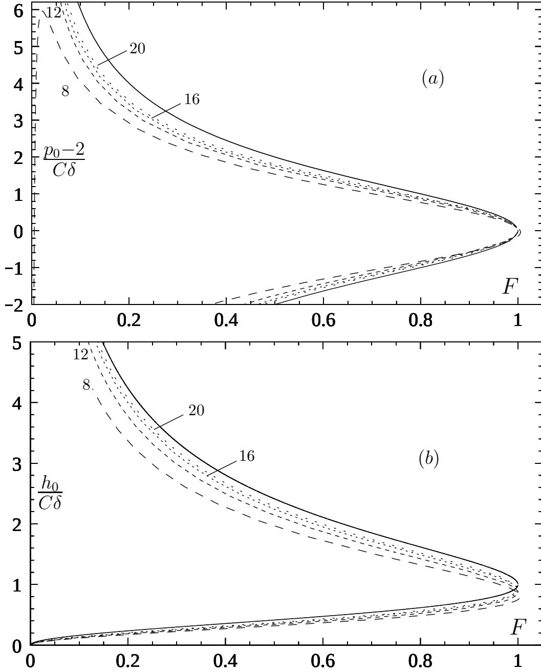
FIGURE 9. Broken curves, numerical solutions of (3.3) for the value of -\log_{10}(CrJa) indicated by the label on each curve. Solid curve, (9.2). C is defined by (7.8); and \delta , by (6.2). The upper branch of the curve for h_0 corresponds to the lower branch of that for p_0 ; for these states, equilibrium of a freely floating sphere is stable. In figure 7b, only the solid curve is concave down as F \rightarrow 0 .
