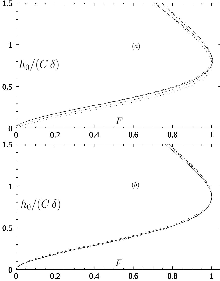
FIGURE 10. Result of evaluating the asymptotic series (9.3b) to various orders for Ja Cr = 10^{-8} (figure (a)) and 10^{-12} (figure (b)): to O(\lambda) , - - - ; to O(\lambda^2) , - \cdot - ; to O(\lambda^3) , \cdots . Solid curves: corresponding values obtained from numerical solutions of (3.3).
