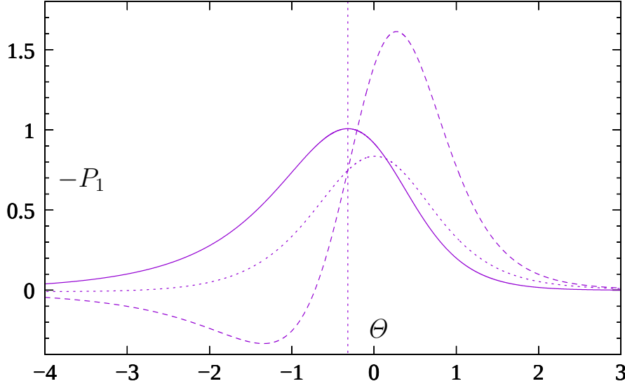
FIGURE 7. Solid curve, -P_1 = H_1'' for \beta = \frac{1}{2}\pi ( \tau = 0.23577 ). Broken curves, Contributions to the gradient -P_1' in perturbation pressure (not to -P_1 itself) are also shown: Q_1/H_0^3 ( \cdots ); 3H_1/H_0^4 ( - - - ). Vertical line, location at which Q_1 = 3H_1/H_0 and -P_1' = 0 .
