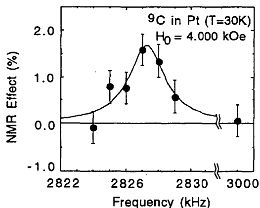
Figure 1. NMR spectrum of ^9\text{C} in Pt
