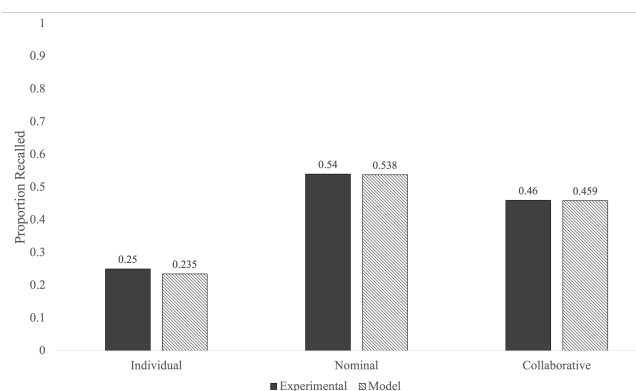
Figure 3. SAM model fit to categorized list data from B. H. Basden et al. (1997). Subjects in groups of 3 were asked to recall from a list of 90 words grouped into 6 total categories with 15 items in each category. The larger category size results in a more prominent collaborative inhibition effect.
