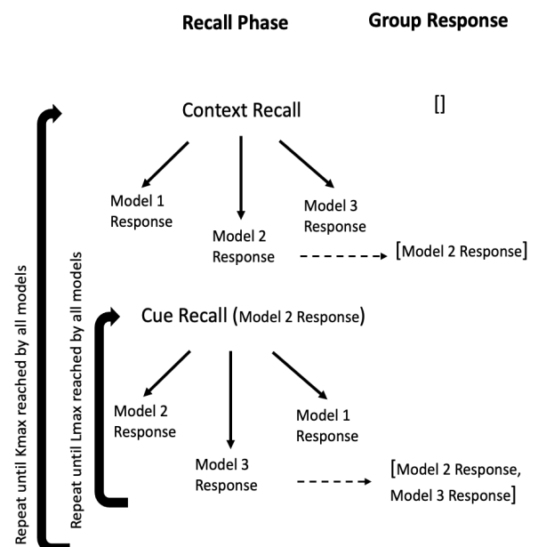
Figure 1. Flowchart of collaborative recall between two or more SAM models.
