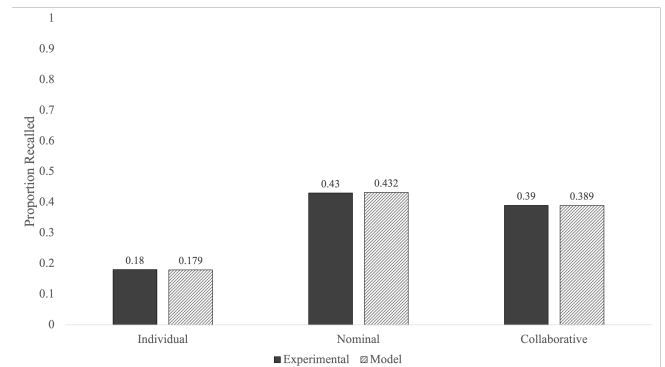
Figure 4. SAM model fit to categorized list data from B. H. Basden et al. (1997). Subjects in groups of 3 were asked to recall from a list of 90 words grouped into 15 total categories with 6 items in each category. The smaller category size results in a less prominent collaborative inhibition effect.
