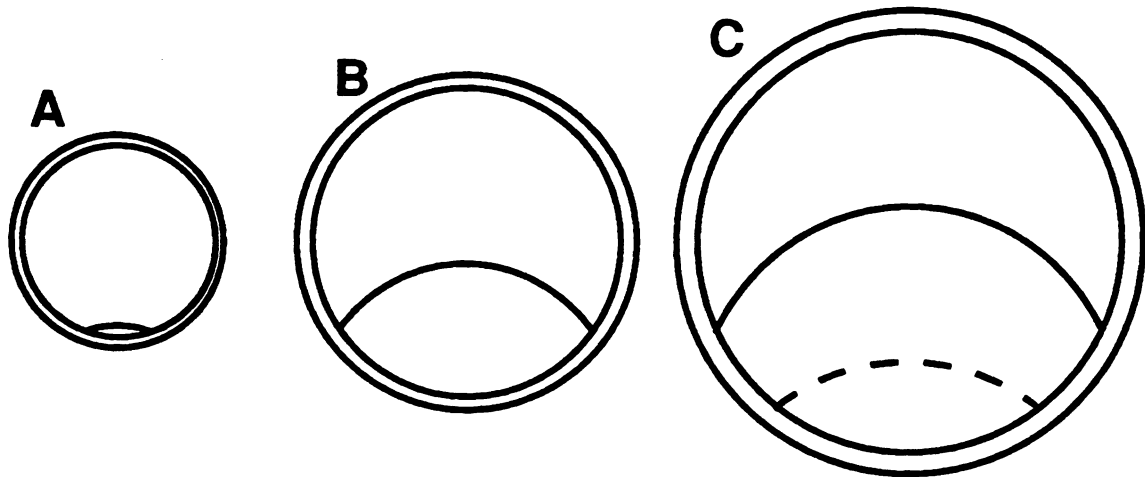
Figure 6: Isotherm curves ( \Delta T=55^\circ\text{C} ) in vessels of various diameters ( d ) and incident energy densities ( D ). A: d=50 \mu\text{m} and D=3 \text{ Jcm}^{-2} ; B: d=80 \mu\text{m} and D=3 \text{ Jcm}^{-2} ; C: d=110 \mu\text{m} and D = 3 (—) or 5 (---) \text{Jcm}^{-2} .
