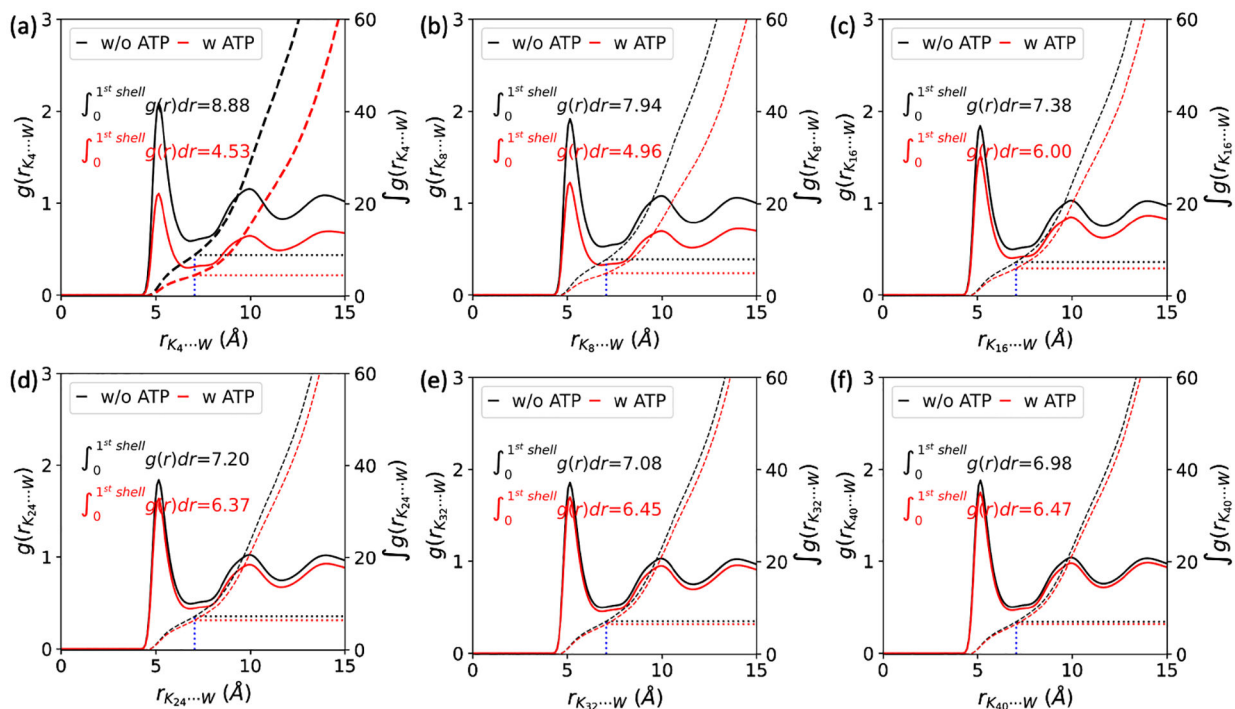
Fig. 3. The radial distribution function formed between oligolysines of different lengths ( K_4 , K_8 , K_{16} , K_{24} , K_{32} , and K_{40} ) and water beads (W), with (red line) or without (black line) the addition of ATPs at the ionic concentration of 0.15 M. Together shown are their corresponding integrations in dashed lines and the number of water beads in the first shell.
