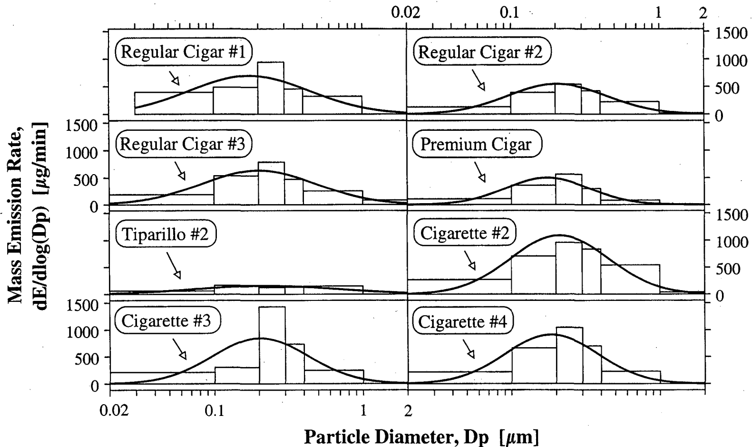
Figure 5: The estimated size distribution of particle mass emission rate (in \mu\text{g}/\text{min} ) and the corresponding log-normal fits for eight experiments. The text in each panel gives the type of source used in each experiment. See Table 1 for the fitted mass median diameter ( MMD ), geometric standard deviation ( GSD ), and integrated mass emissions. The average MMD and GSD were 0.20 \mu\text{m} and 2.3, respectively.
