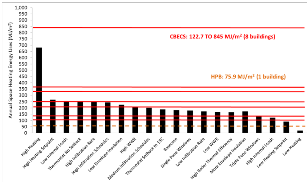
Figure 11. Benchmarking simulation results with the building databases for the small office building in Minneapolis.
