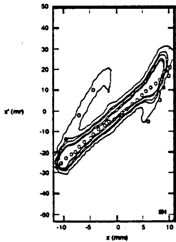
Fig. 1 Measured beam distribution in (x, x') phase space at diode exit. Comparison between experiment (-) and EGUN (o). Upper (lower) figure refers to the new (old) source.
