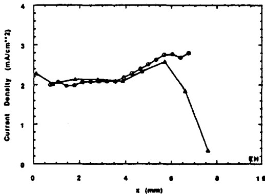
Fig. 4 5 mA beam current density at point of injection into first quadrupole of matching section. Comparison between experiment ( \Delta ) and EGUN code ( \bullet ).
