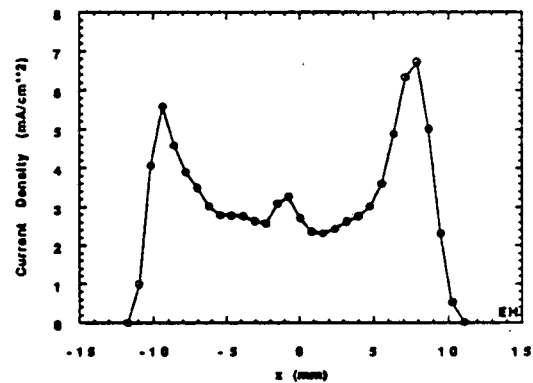
Fig. 2 Measured beam current density distribution vs. radial position. Upper (lower) figure refers to the new (old) source.
