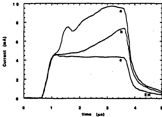
Fig. 3 Scraped beam current vs. time with a scraper bias of (a) 0.75kV, (b) 2.75 kV and (c) 4.75 kV.
