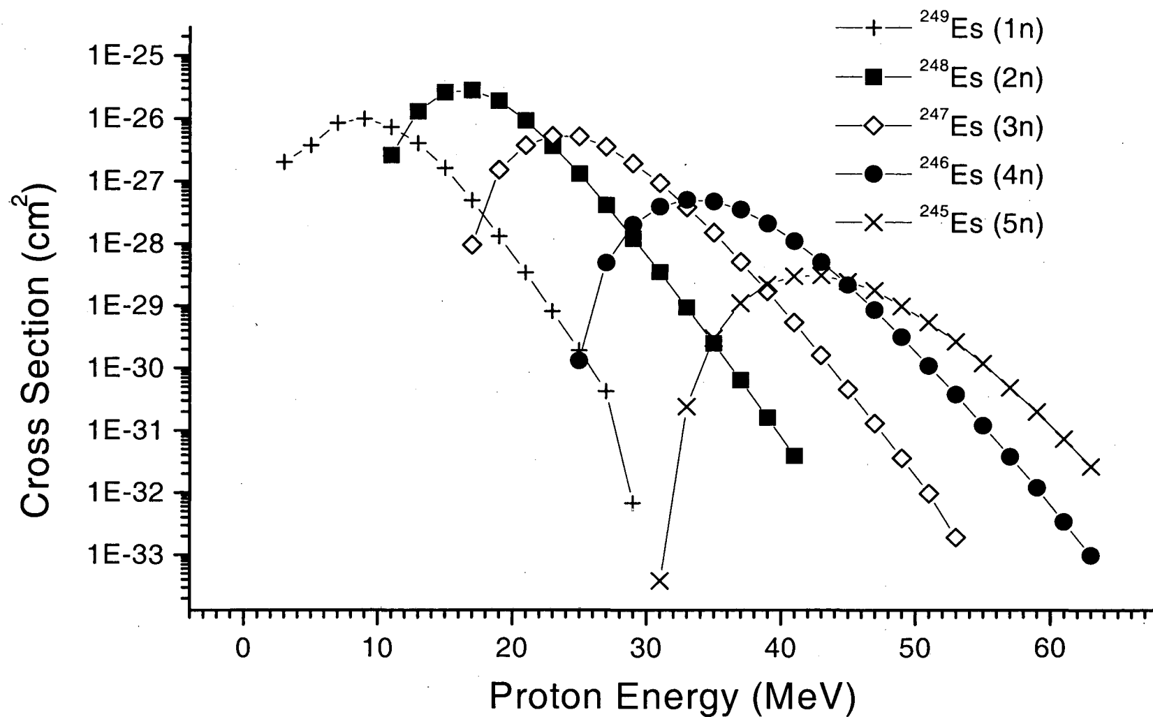
Figure 4.8: Predicted cross sections for the production of einsteinium isotopes using the ^{249}\text{Cf}(p,xn)^{250-x}\text{Es} reaction. Cross sections were determined using the SPIT [SIK67] code.
