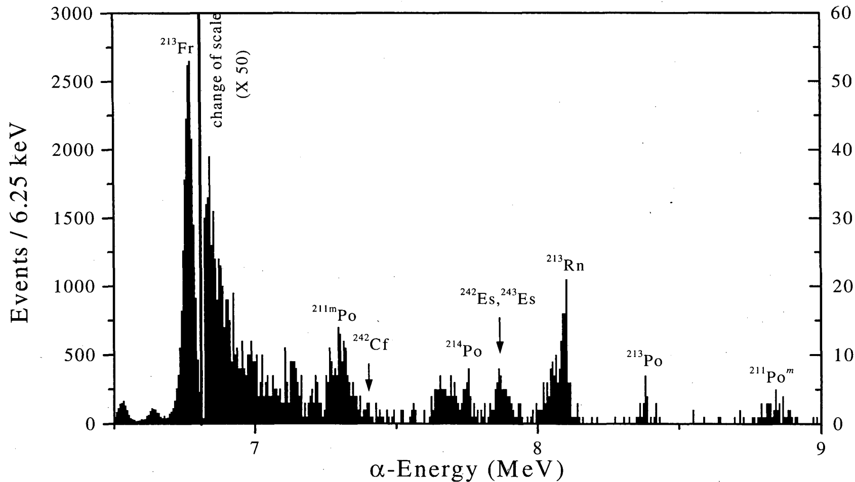
Figure 6.4: Summed \alpha -spectrum for the ^{233}\text{U}(^{14}\text{N},\text{xn})^{247-\text{x}}\text{Es} reaction at 87 MeV. This spectrum was the sum of all data recorded while the MG was stepping during the third ^{242}\text{Es} ECDF experiment (48 h of beam time.) Note the change of scale between the ^{213}\text{Fr} peak and the rest of the spectrum.
