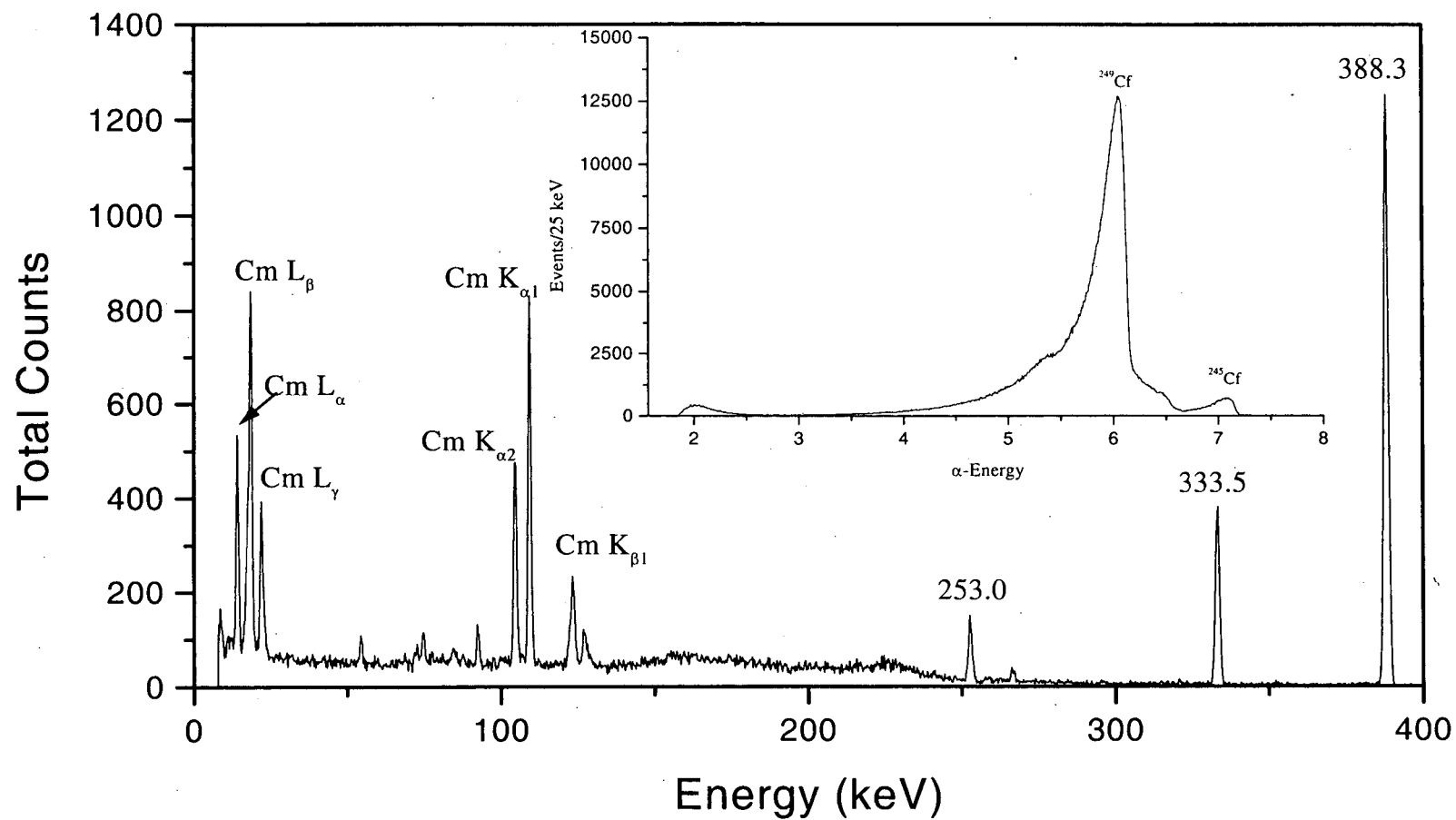
Figure 6.14: Sample x-ray and \alpha -spectra from the x-ray/fission coincidence setup at 37 MeV.
