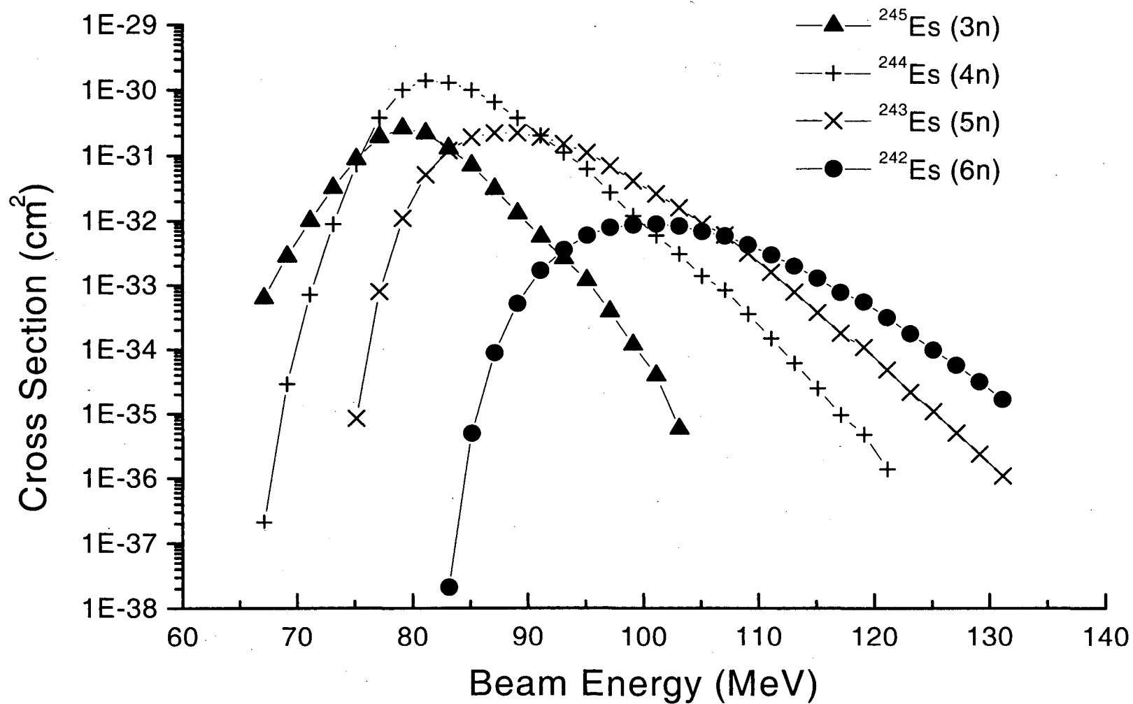
Figure 4.6: Predicted cross sections for the production of einsteinium isotopes using the ^{233}\text{U}(^{15}\text{N}, \text{xn})^{248-\text{x}}\text{Es} reaction. Cross sections were determined using the SPIT [SIK67] code.
