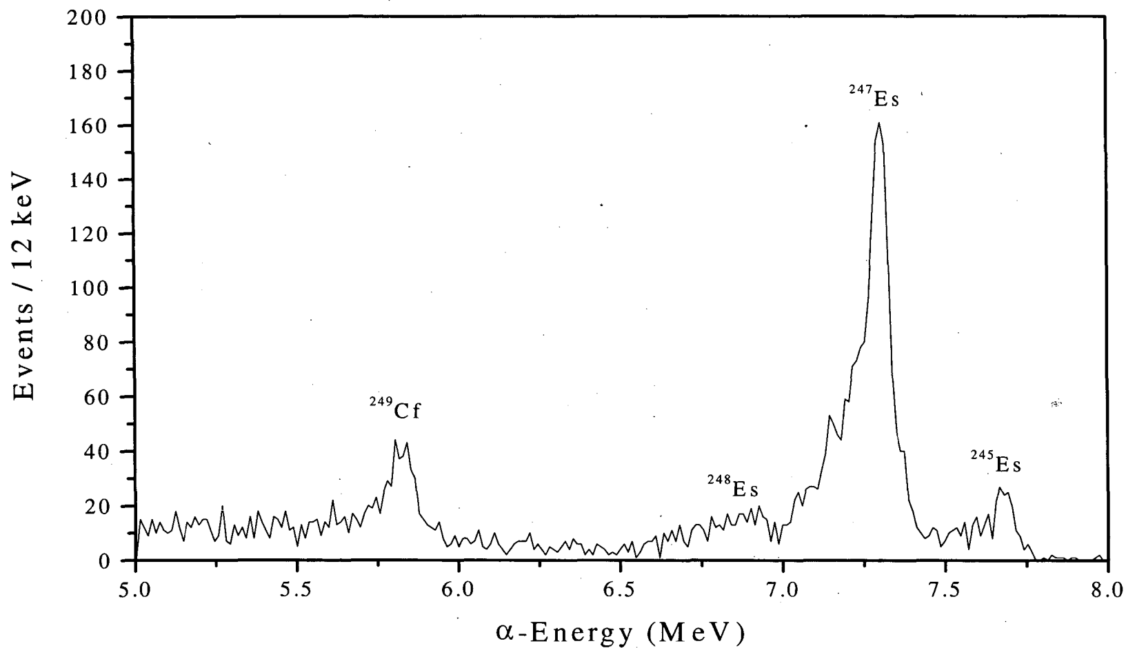
Figure 6.20: \alpha -spectrum from the ^{249}\text{Cf}(\text{p},\text{xn})^{250-\text{x}}\text{Es} reactions at 40 MeV. The spectrum was taken from the top detector of the second detector pair using a 1-min stepping time in the MG (80 min of collection and counting.) The ^{249}\text{Cf} is target material that was knocked out by the beam.
