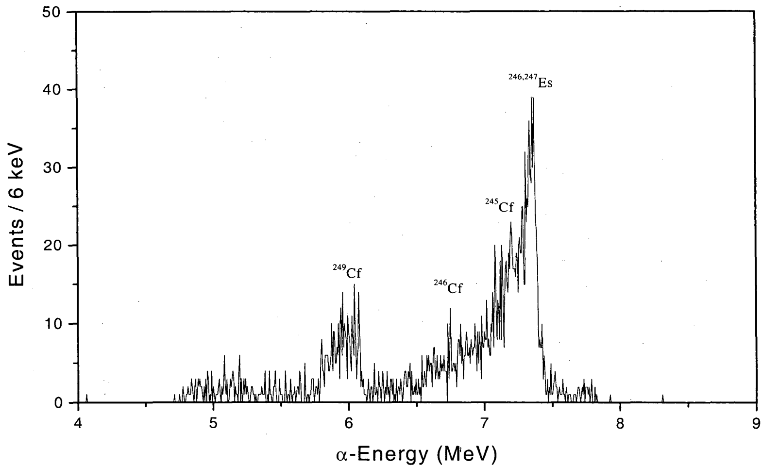
Figure 6.12: \alpha -spectrum from the ^{249}\text{Cf}(p, xn)^{250-x}\text{Es} reaction at 37 MeV. A 1-min stepping interval was used in the MG for a total of 80 min of collection and counting. This spectrum was taken from the top detector of the second detector pair.
