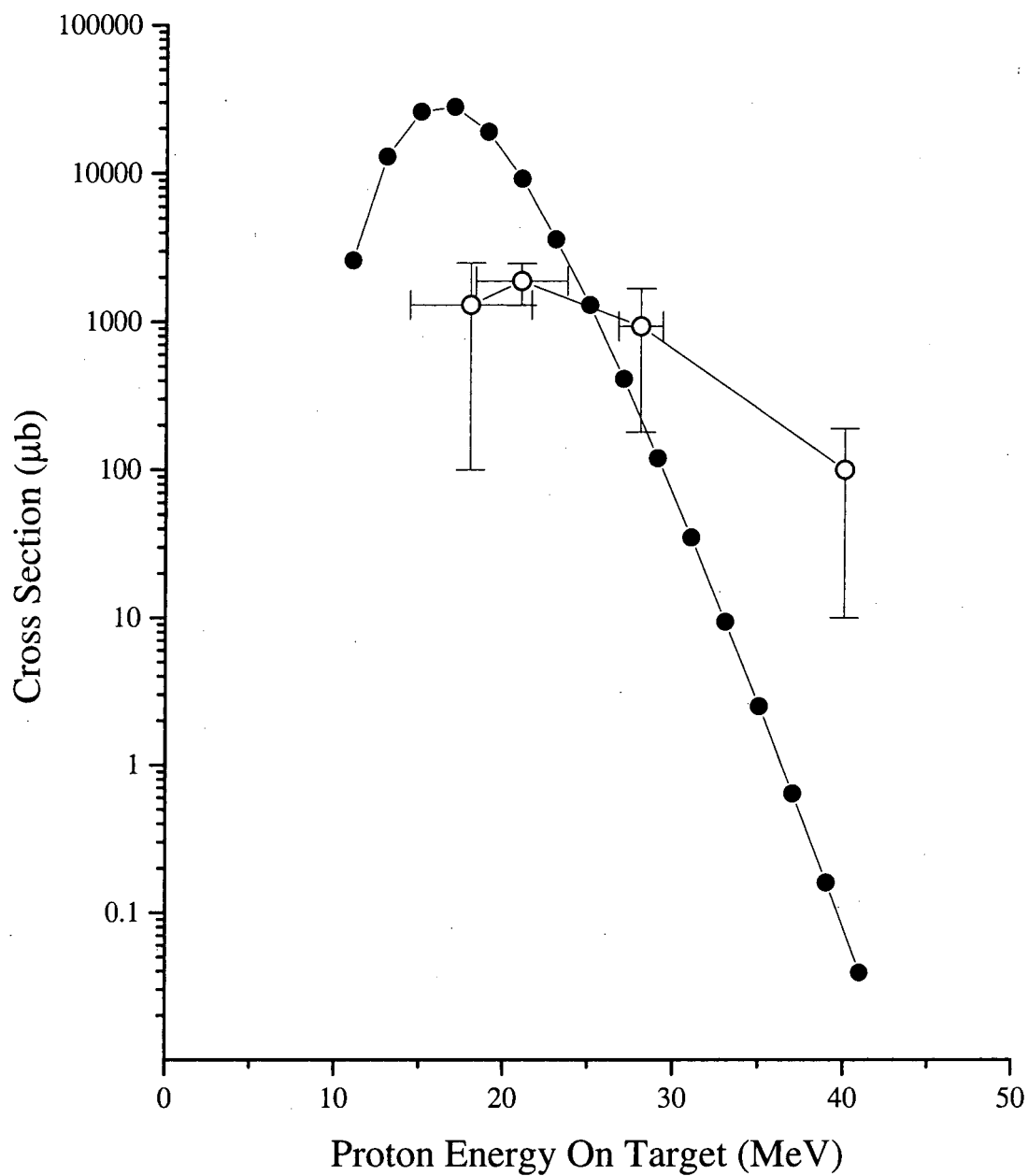
Figure 6.29: Experimentally determined cross sections for the ^{249}\text{Cf}(p,n)^{248}\text{Es} reaction (open circles) and the SPIT predictions (closed circles [SIK67]) for the same reaction.
