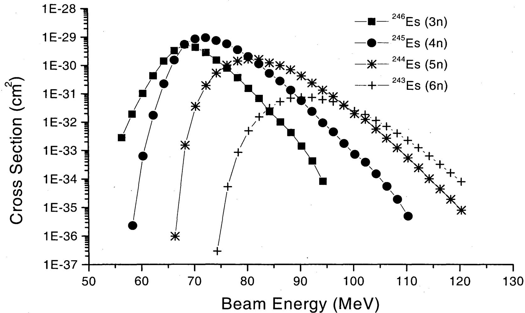
Figure 4.7: Predicted cross sections for the production of einsteinium isotopes using the ^{237}\text{Np}(^{12}\text{C}, \text{xn})^{239-\text{x}}\text{Es} reaction. Cross sections were determined from the SPIT [SIK67] code.
