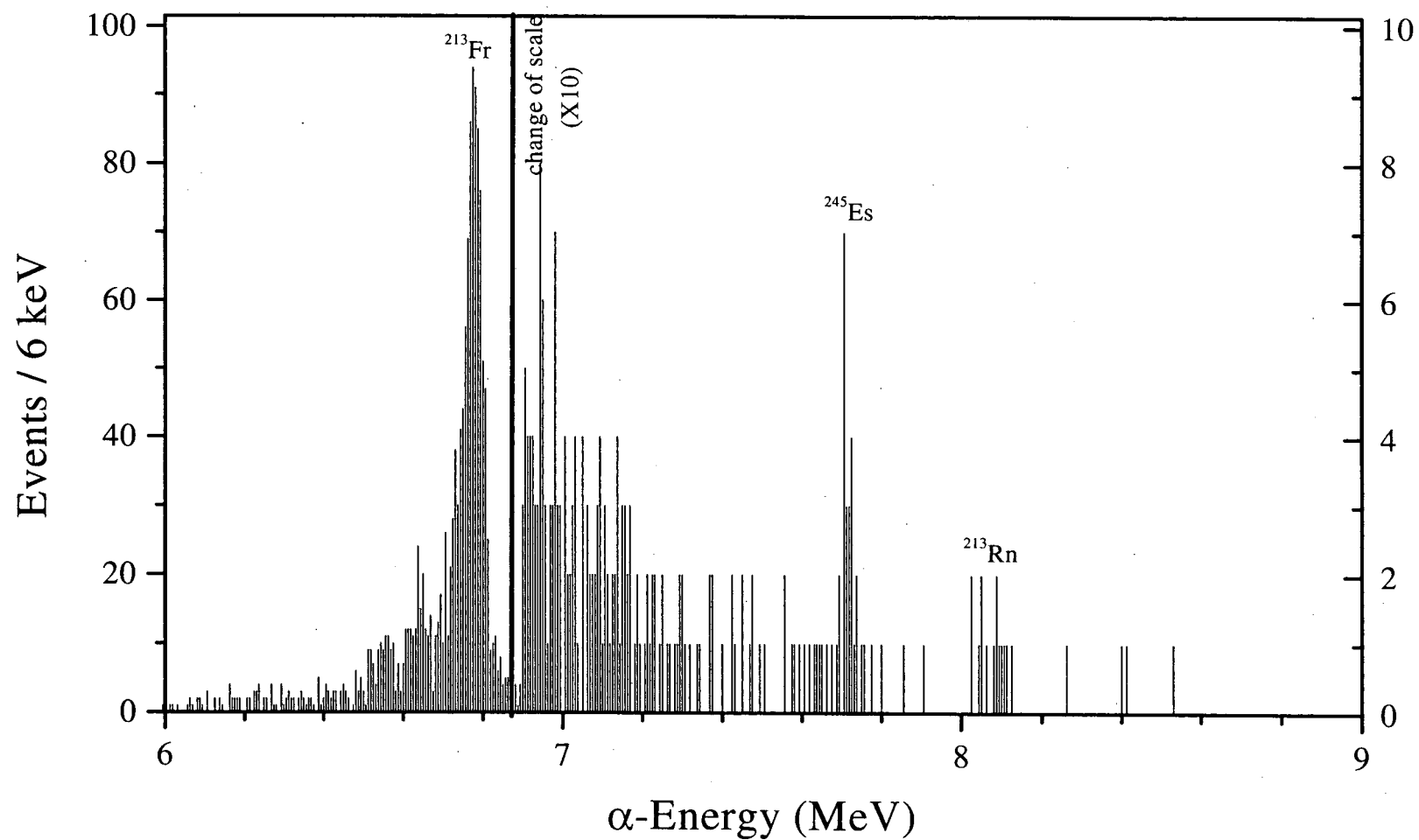
Figure 6.18: \alpha -spectrum from the ^{233}\text{U}(^{15}\text{N},\text{xn})^{248-\text{x}}\text{Es} reaction at 80 MeV. Note the change of scale after the ^{213}\text{Fr} peak. The spectrum was taken from the top detector of the second detector pair using a 1-min stepping interval in the MG, and represents 80 min of collection and counting.
