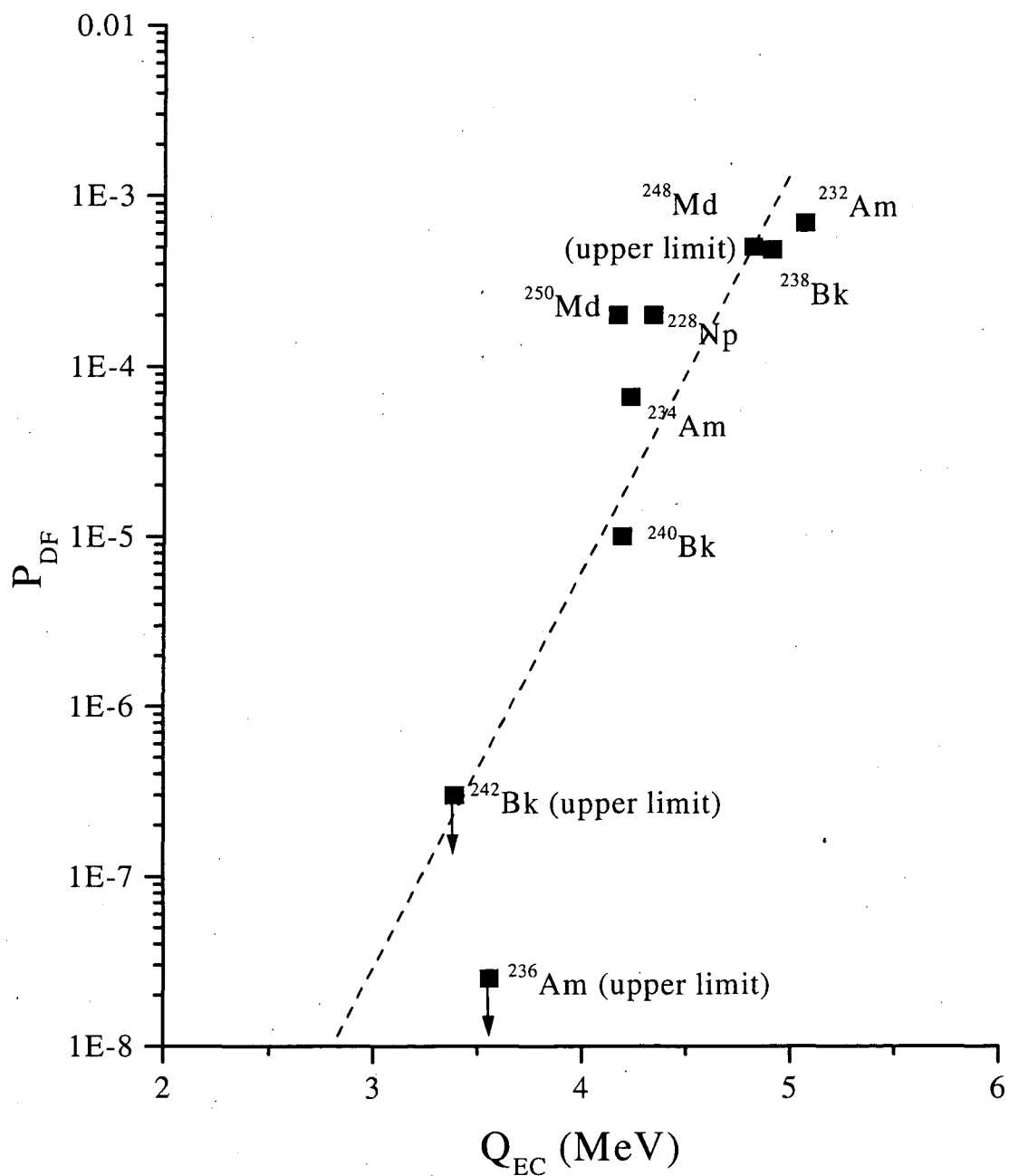
Figure 2.2: Experimentally measured P_{DF} values versus Q_{EC} . Q-values were calculated from the masses in [MÖL95]. Data are from References [GAN80, HAL89, HAL90, HAL90A, KRE94, KRE94A]. The line is to guide the eye and is not meant to be a fit to the data.
