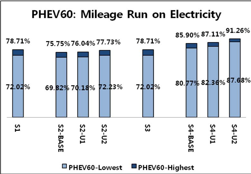
Figure 5.3b Total Mileage Run by Electricity for PHEV 60
