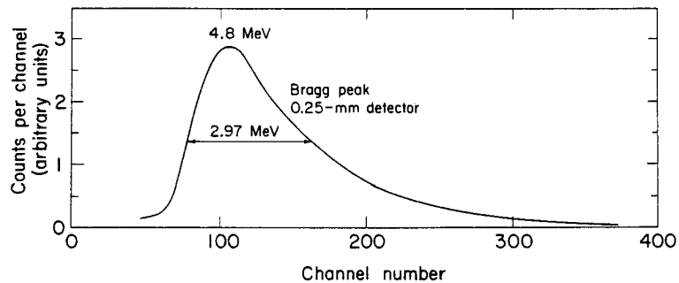
Figure 5. Response of 1/4-mm detector to 910-MeV \alpha beam at the Bragg-peak position. MUB-7542
