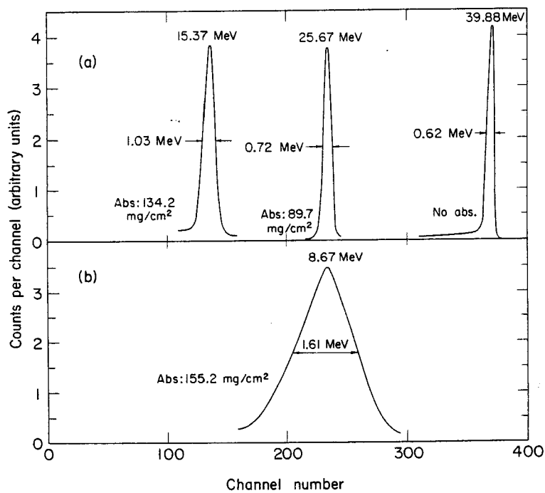
Figure 2. Response of 1-mm detector to 40-MeV \alpha beam and the beam degraded by _2\text{Al} ; (a) 89.7 and 134.2 \text{mg}/\text{cm}^2 _2\text{Al} ; (b) 155.2- \text{mg}/\text{cm}^2 _2\text{Al} . MUB-7539
