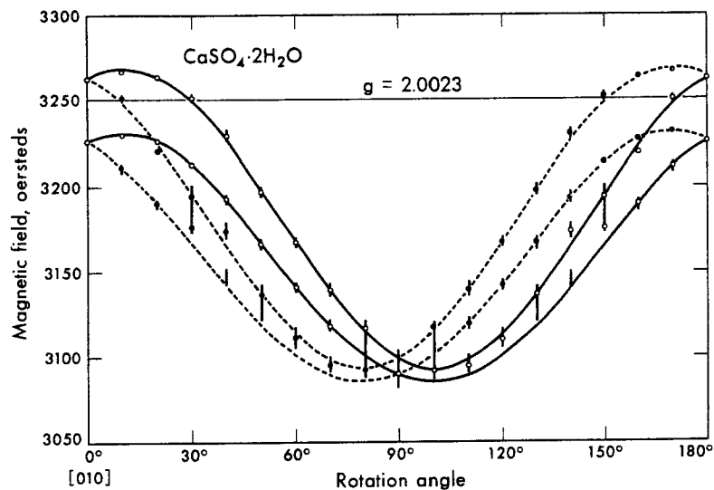
Figure 3. Magnetic field vs rotation angle for electron-irradiated CaSO 4 ·2H 2 O at 77°K. The spin Hamiltonian parameters are g 2.1108, g 2.0028, A 43 Oe, A 32.5 Oe, A 3.3 Oe. MUB-3670
