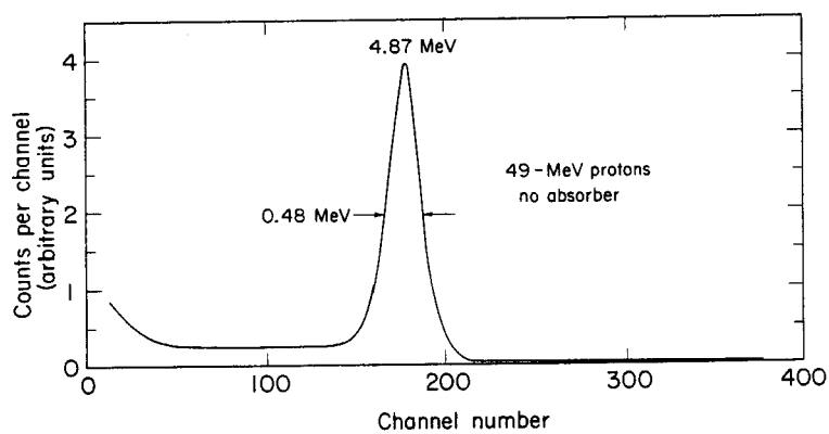
Figure 7. Response of 0.68 g/cm 2 ( \approx 3 mm) detector to 49-MeV proton beam. MUB-7544
