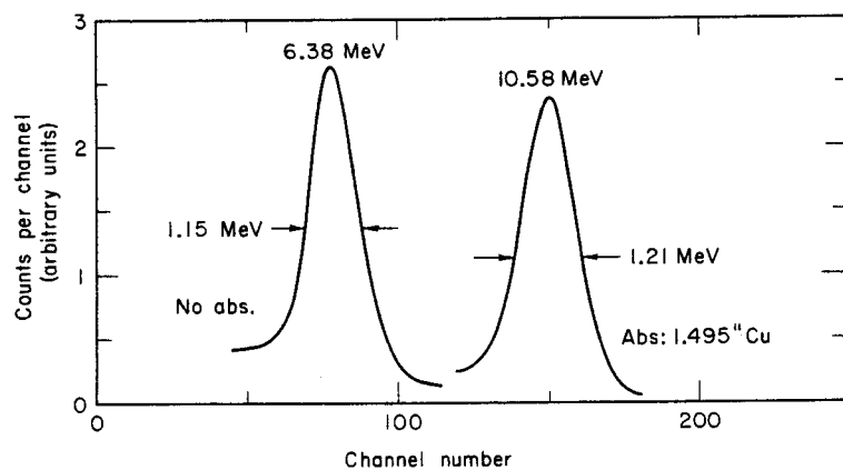
Figure 3. Response of 0.48- \text{g}/\text{cm}^2 ( \approx 2\text{mm} ) detector to 910-MeV \alpha beam, and the beam degraded by 1.495 in. cu. MUB-7540
