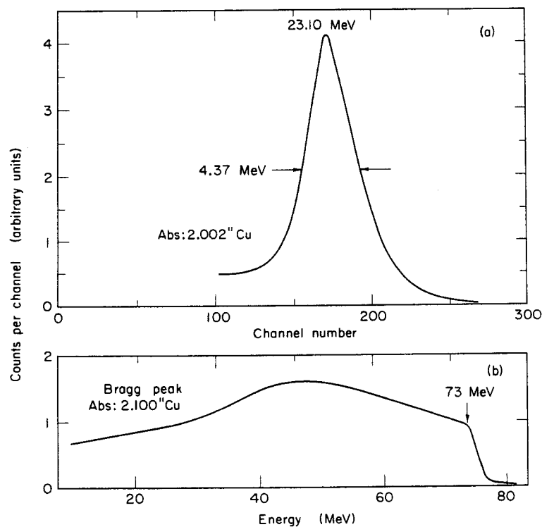
Figure 4. Response of 0.48- \text{g}/\text{cm}^2 ( \approx 2\text{mm} ) detector to 910-MeV \alpha beam degraded by (a) 2.002 in. cu; (b) 2.100 in. cu (Bragg peak). MUB-7541
