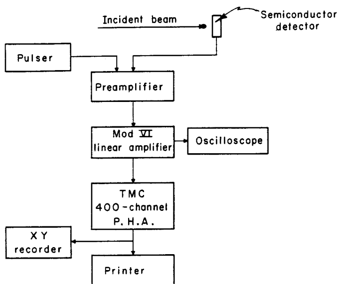
Figure 1. Experimental setup. MUB-4136A
