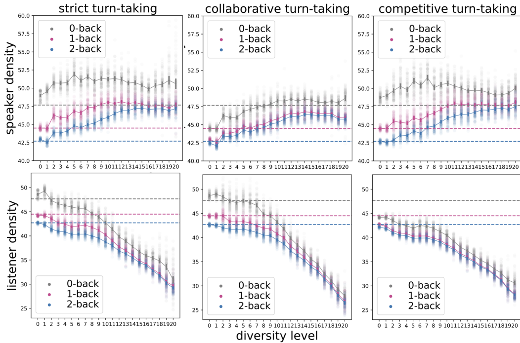
Figure 4: Speaker and listener density for all turn-taking protocols and n-back conditions. Experiment 1 are the grey line (0-back) in the left panels (strict turn-taking) protocols. Results for Experiment 2 are the grey lines (0-back results) across all turn-taking protocols. Results for Experiment 3 encompass all data displayed in the graph. Dashed lines represent values from individual performance.
