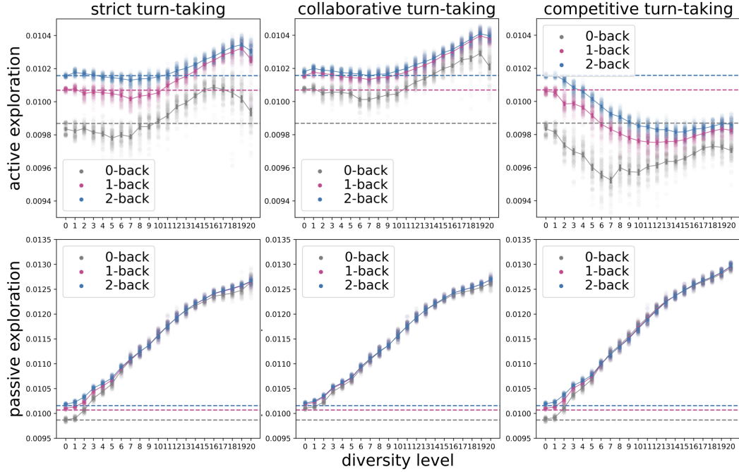
Figure 3: Active exploration and passive exploration across all turn-taking protocols and n-back conditions. Results for Experiment 1 are the grey line (0-back) in the left panels (strict turn-taking) protocols. Results for Experiment 2 are the grey lines (0-back) across all turn-taking protocols. Results for Experiment 3 encompass all data displayed in the graph. Dashed lines represent values from individual performance.
