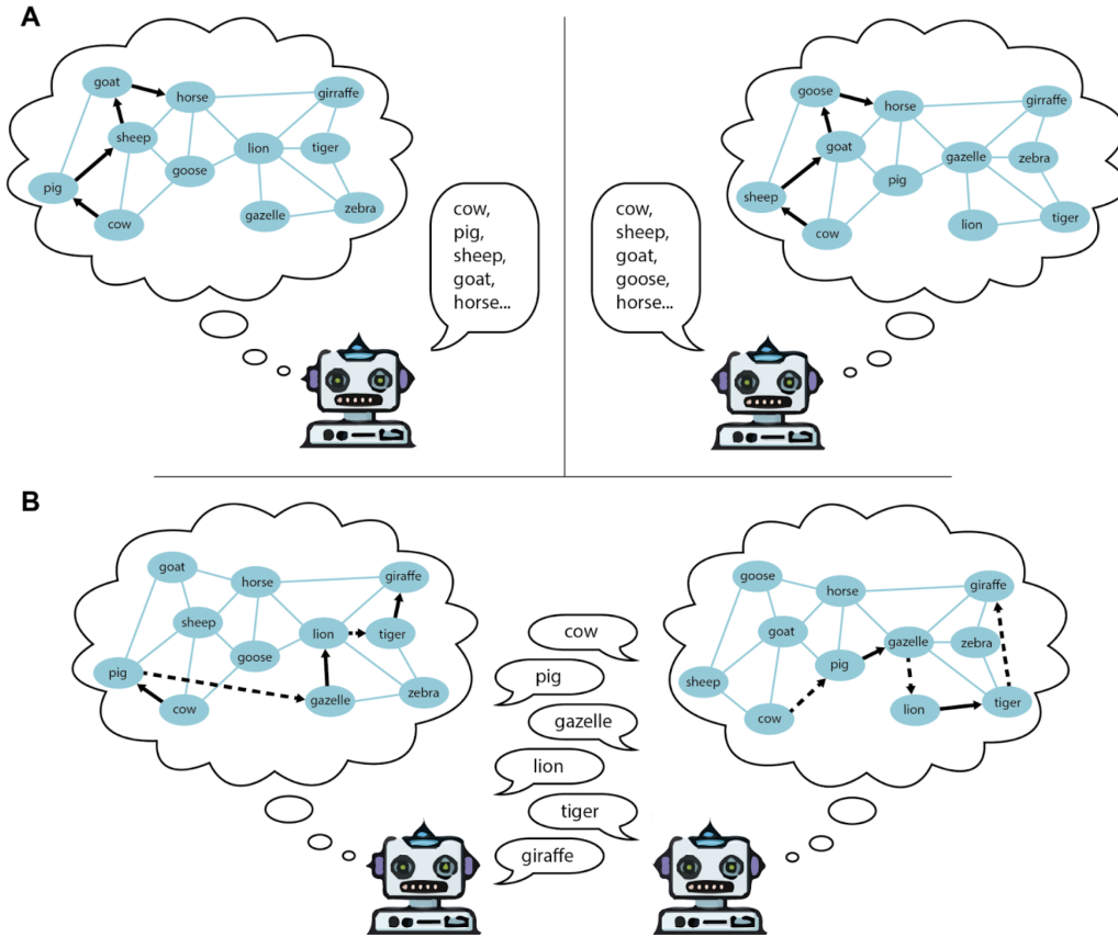
Figure 1: Schematic depiction of the simulation mechanics. A: Two agents performing the verbal fluency task individually. B: The same two agents doing the task collectively. As in the individual condition, the turn-holder names the animal closest to the previously named animal. Yet, as since agents vary in their semantic memories, the resulting trajectories through semantic space are different than what individual agents would produce. Black arrows represent associations made by the agent, dashed arrows are associations made by the partner.
