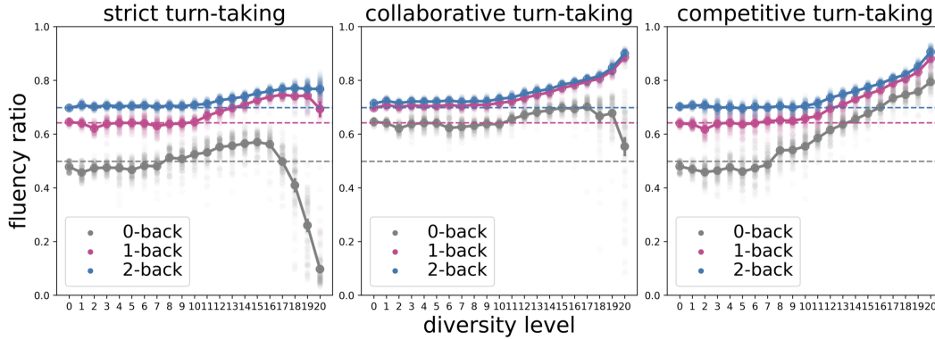
Figure 2: Fluency ratio (average proportion of animals named across simulations by each pair) across turn-taking protocols and n-back conditions in all experiments. Results for Experiment 1 are the grey lines, labelled as 0-back, in the strict turn-taking protocols . Results for Experiment 2 are the grey lines (0-back) across all turn-taking protocols . Results for Experiment 3 encompass all data displayed in the graph. Dashed lines represent the fluency ratios in individual simulations.
