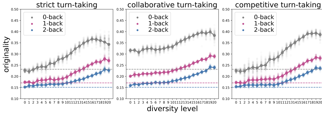
Figure 5: Originality across turn-taking protocols and n-back conditions in all three experiments. Dashed lines represent individual performance. Results for Experiment 1 are the 0-back results in the strict turn-taking protocols. Results for Experiment 2 are the 0-back results across all turn-taking protocols. Results for Experiment 3 encompass all data displayed in the graph.
